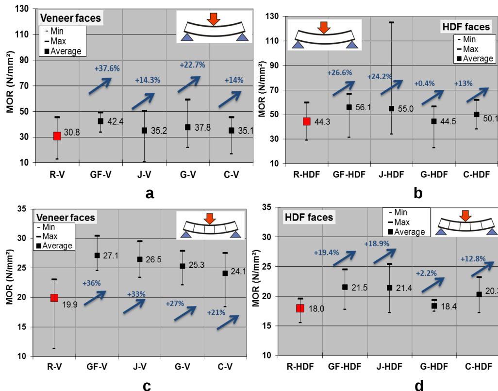
Fig. 4. MOR values: a) MOR // and veneer faces, b) MOR// and HDF faces, c) MOR⊥ and veneer faces, and d) MOR⊥ and HDF faces
