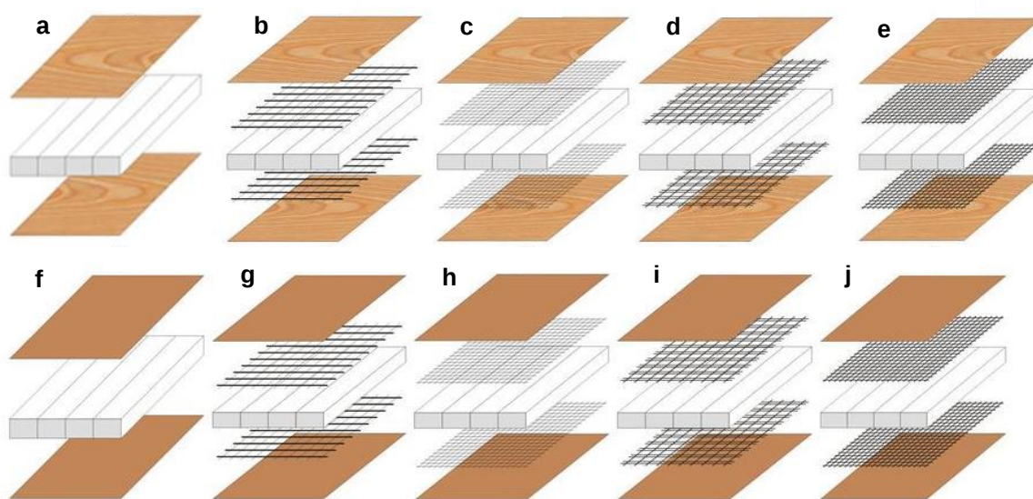
Fig. 2. Design of the manufactured blockboard structures: a) R-V; b) GF-V; c) G-V; d) J-V; e) C-V; f) R-HDF; g) GF-HDF; h) G-HDF; i) J-HDF, and j) C-HDF
