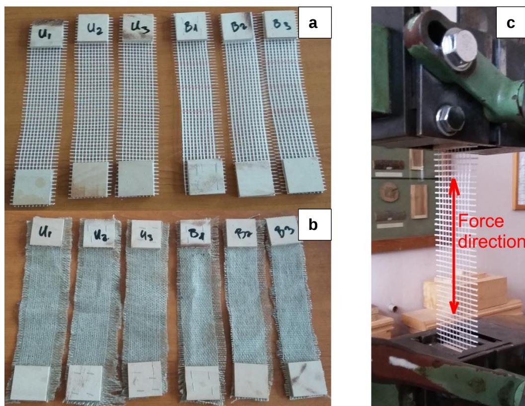
Fig. 1. Specimens prepared for the tensile strength test; a) glass fiber; b) jute fabric, and c) performance of the tensile test at the universal testing machine
