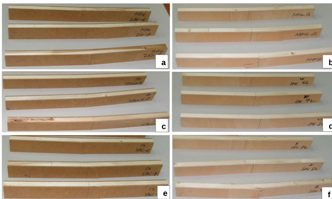
Fig. 7. Failure modes of specimens during bending test parallel to the core grain orientation: a) R-HDF, b) R-V, c) GF-HDF, d) GF-V, e) J-HDF, and f) J-V
