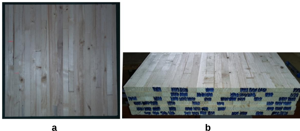
Fig. 6. Blockboard's spruce core; a) the core area with strips jointed end to end and b) marked rows where strips with small lengths are jointed end to end
