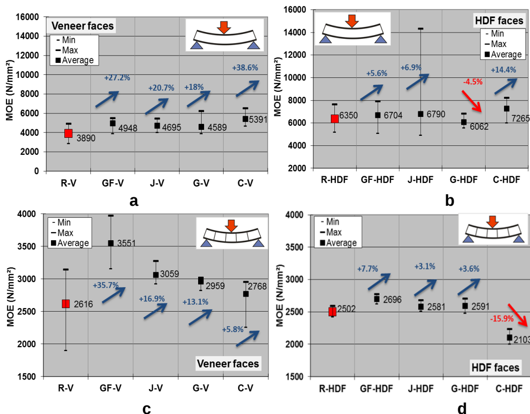
Fig. 5. MOE values: a) MOE // and veneer faces, b) MOE // and HDF faces, c) MOE ⊥ and veneer faces, and d) MOE ⊥ and HDF faces
