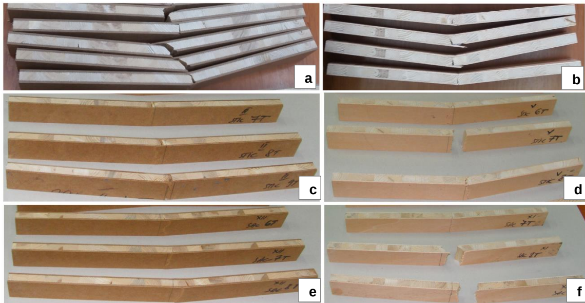
Fig. 8. Failure modes of specimens during bending test perpendicular to the core grain orientation: a) R-HDF, b) R-V, c) GF-HDF, d) GF-V, e) J-HDF, and f) J-V
