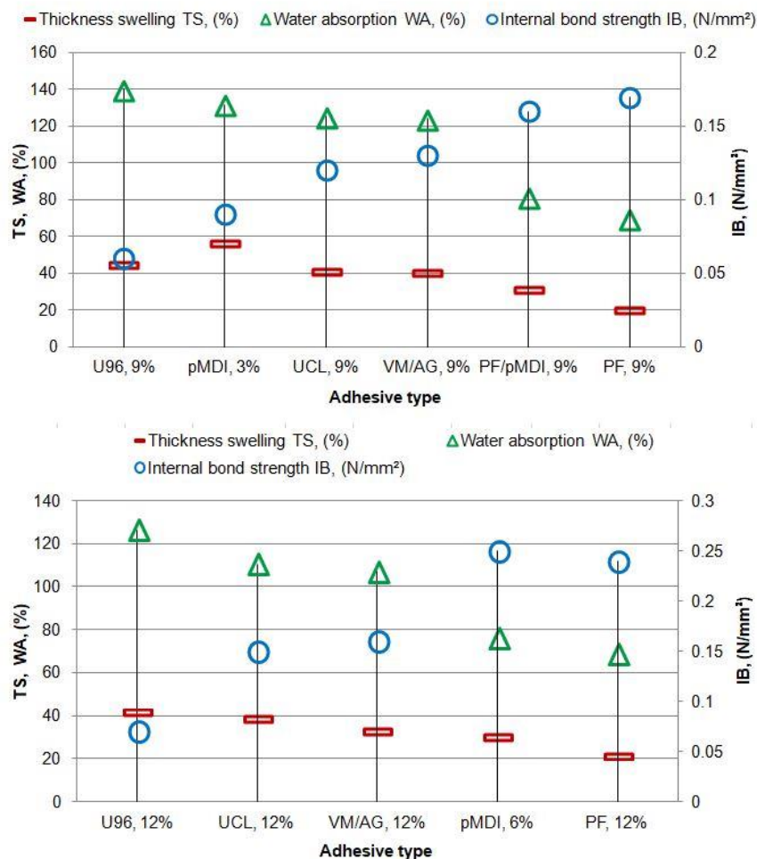
Fig. 4. Effect of adhesive type and its content level on the thickness swelling (TS), water absorption (WA), and internal bond strength (IB) of the panels
