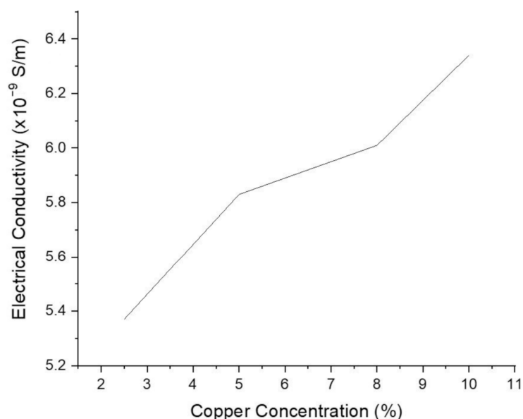
Figure 19. Electrical conductivity of copper-reinforced polymer composites.
