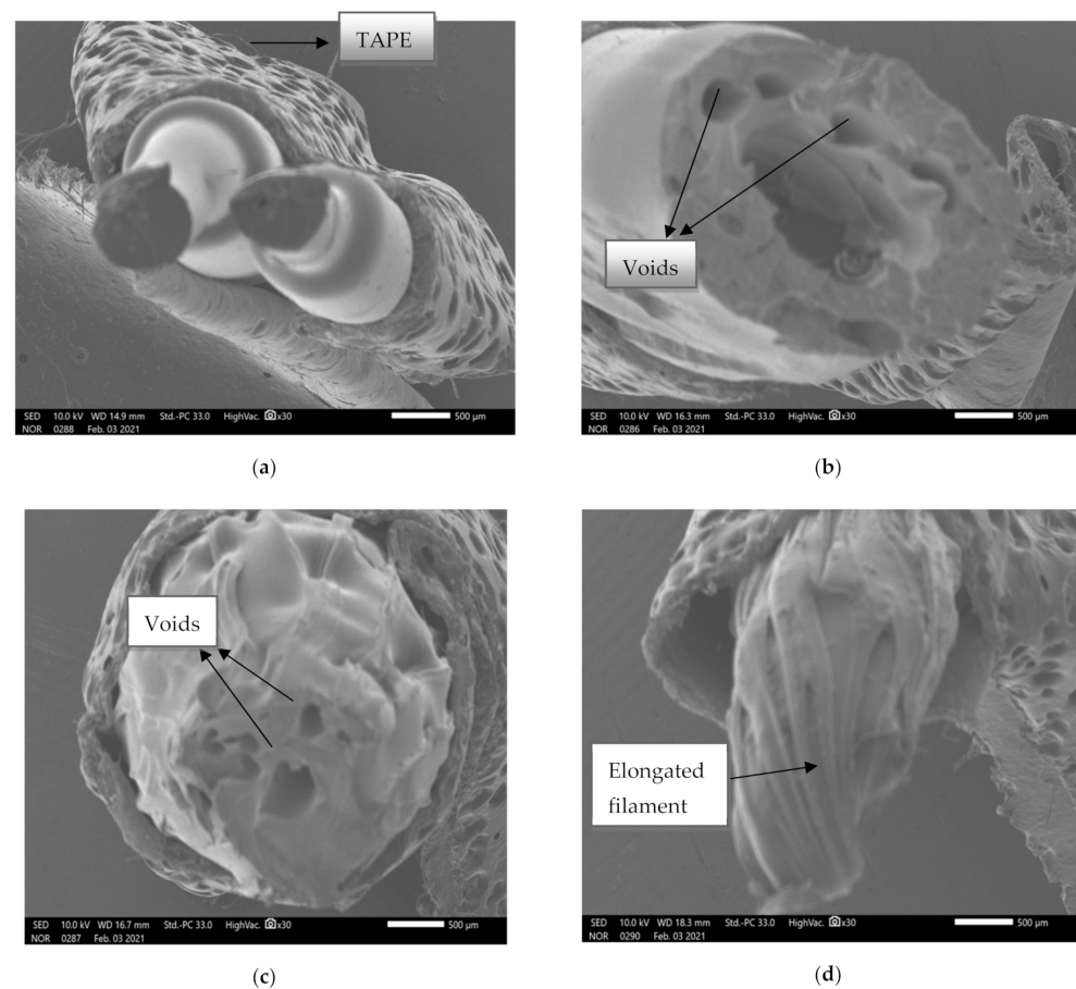
Figure 18. SEM Images of (a) C2, (b) B4, (c) B10, and (d) C8.
