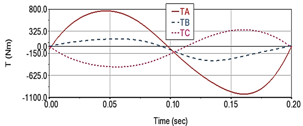
Figure 6. Driving torques ( T_A , T_B and T_C ) for the Delta robot reference model.
