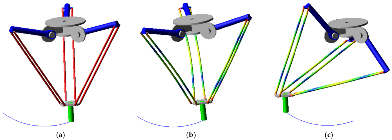
Figure 8. The CAD model of the Delta robot: (a) in ideal case, and with flexible links at (b) trajectory start point P_0 ; (c) trajectory end point P_1 .
