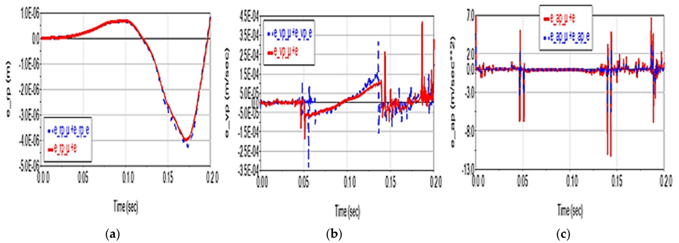
Figure 14. Motion deviations in Scenario 4 (red solid line) and the additive effect of friction and elasticity factors (blue dashed line) for (a) displacement; (b) velocity and (c) acceleration.
