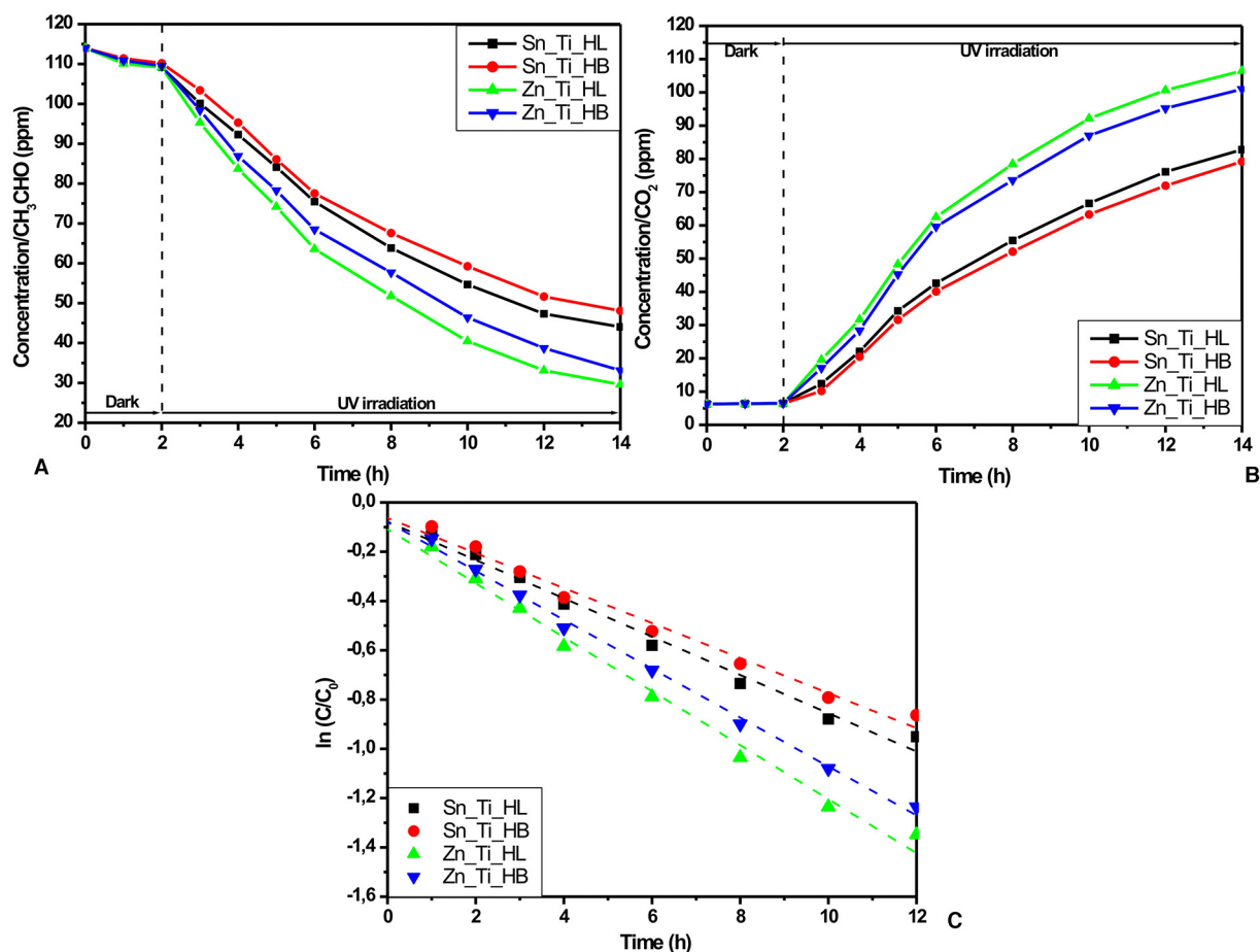
FIGURE 3 | Photocatalytic activity in gaseous environment: (A) amount of CH 3 CHO, (B) amount of CO 2 , and (C) the kinetics of CH 3 CHO photocatalytic degradation using the Langmuir-Hinshelwood correlation.
