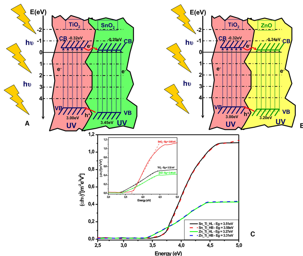
FIGURE 4 | Energy levels diagrams of (A) Sn-Ti, (B) Zn-Ti, and (C) the tandem structures band gap evaluation (inset band gap of the single components).
