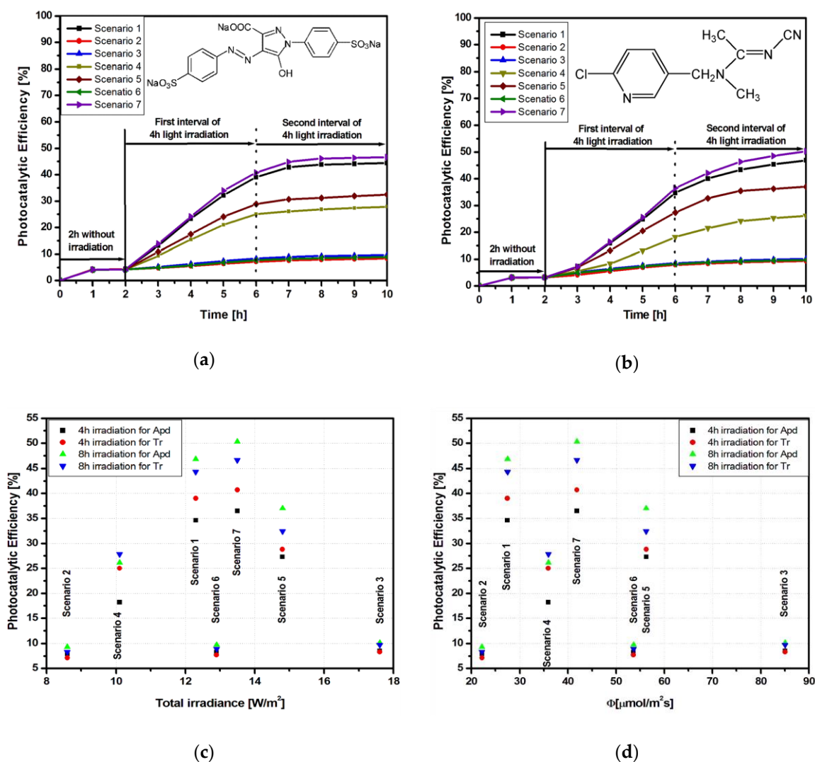
Figure 3. Photocatalytic parameters of the Ti 2 G sample: (a) tartrazine (Tr) photodegradation; (b) acetamidiprid (Apd) photodegradation; (c) total irradiance vs. photocatalytic efficiency, and (d) photon flux vs. photocatalytic efficiency.
