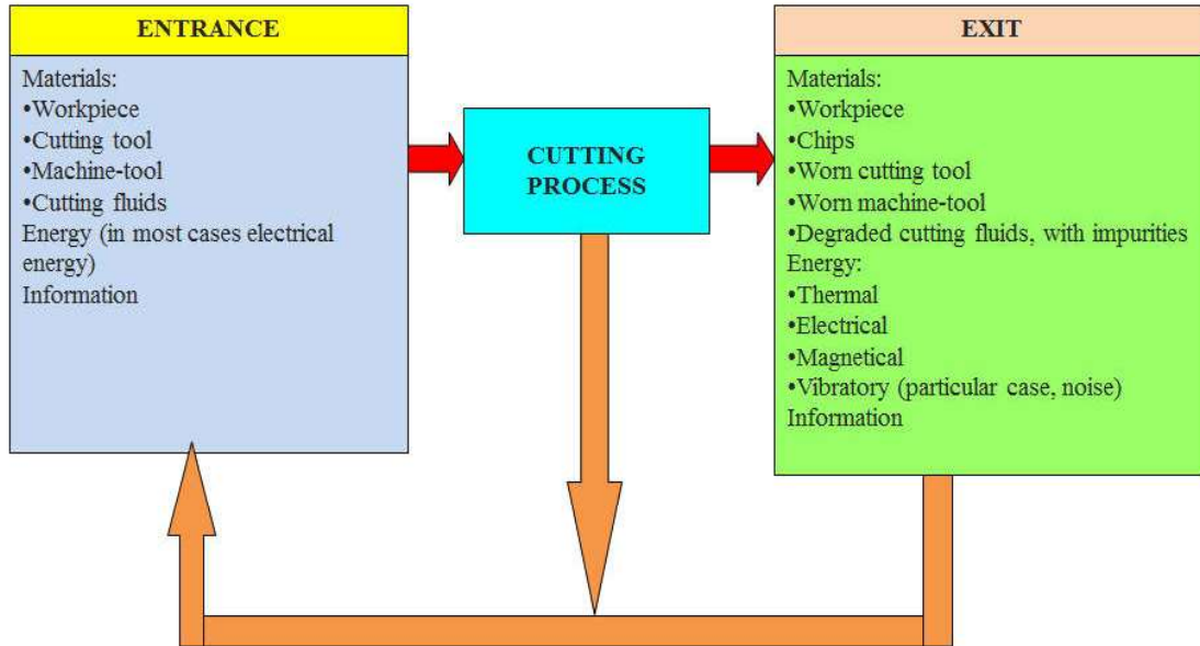
Figure 1. Cutting process as a system.
