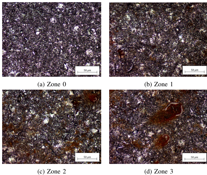
Fig. 11. Microscopic image of the areas defined in Fig.10.
