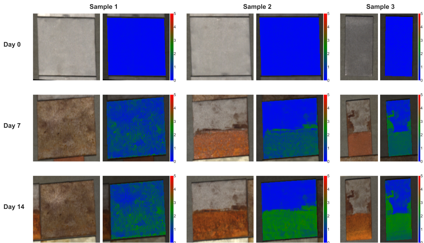
Fig. 9. RGB images and CSI colour map of OC Samples.
