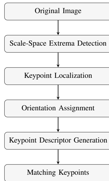
Fig. 6. Flowchart of the SIFT Algorithm.
