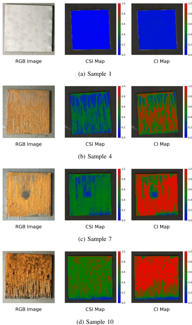
Fig. 13. RGB image, CSI colour map and CI colour map respectively
