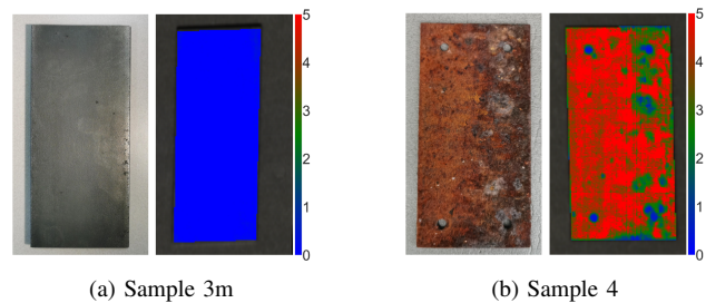
Fig. 12. RGB images and CSI colour map of OC Samples.
