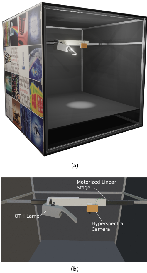
Fig. 5. Experimental setup for hyperspectral measurements [65]. (a) 3D model of the acquisition system. (b) Detailed view of the main components.
