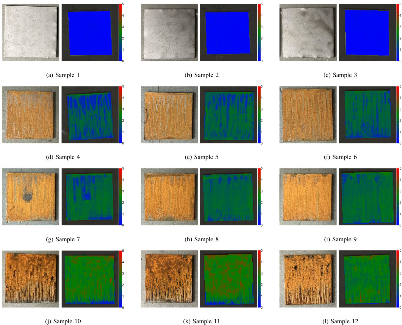
Fig. 8. RGB images and CSI colour map of SSC Samples.
