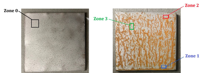
Fig. 10. The zones defined in the samples. On the left, sample without corrosion; on the right, sample exposed for 20 minutes in a salt spray chamber.
