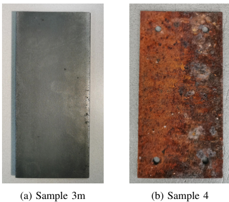
Fig. 4. RGB images of OC Samples.
