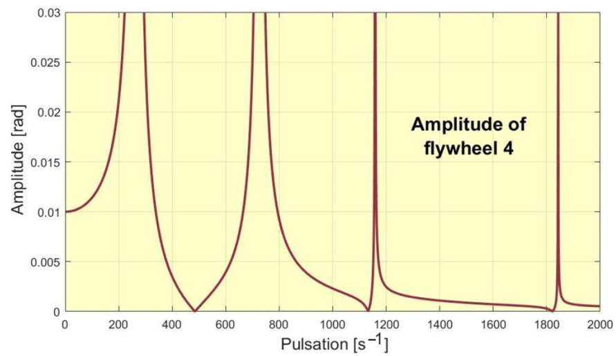
Figure 12. The absorbtion of the flywheel 4 for the simplified system.
