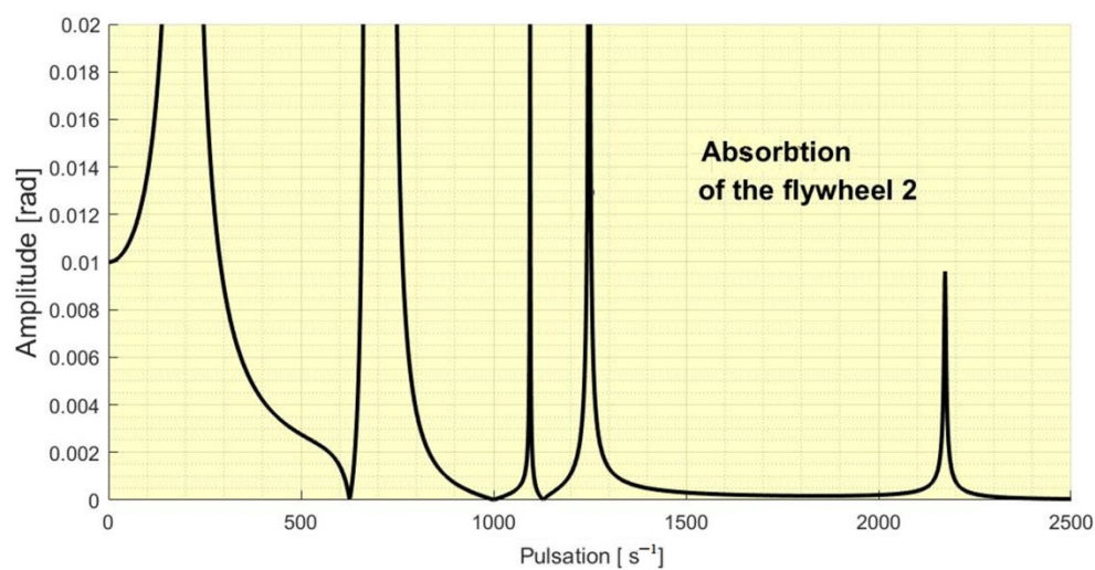
Figure 7. The absorbtion of the flywheel 2.
