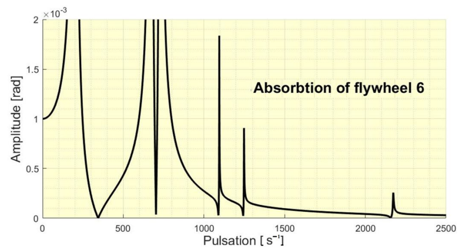
Figure 3. The absorption of the flywheel 6.
