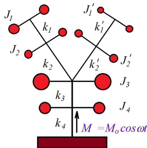
Figure 1. Elastic system with wheels.
