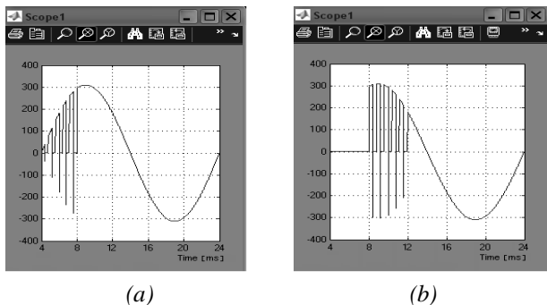
Figure 7. Simulation results in case of supply coupling at AC voltage zero crossing (a) and at AC voltage peak (b)
