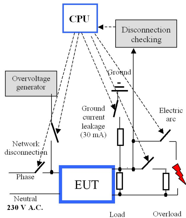
Figure 1. Test bench – Simplified block scheme
