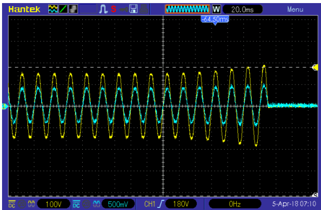
Figure 8. Load disconnection upon the appearance of an overvoltage
