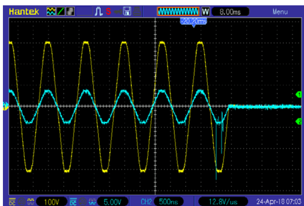
Figure 10. Load disconnection upon the appearance of an electric arc
