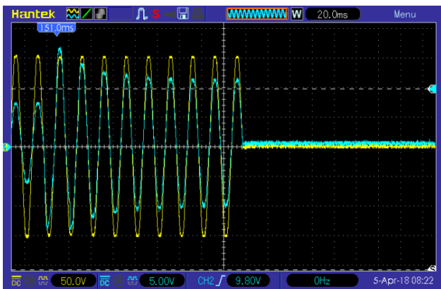
Figure 9. Load disconnection upon the appearance of overcurrent
