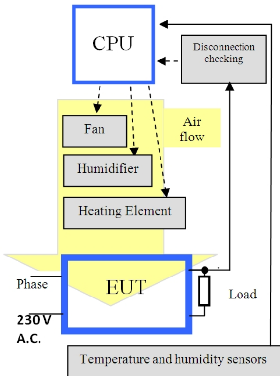
Figure 7. Test bench – Reliability assessment
