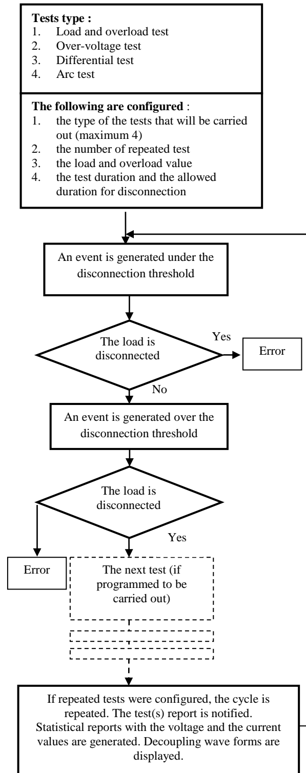
Figure 2. Test bench – Simplified operation diagram
