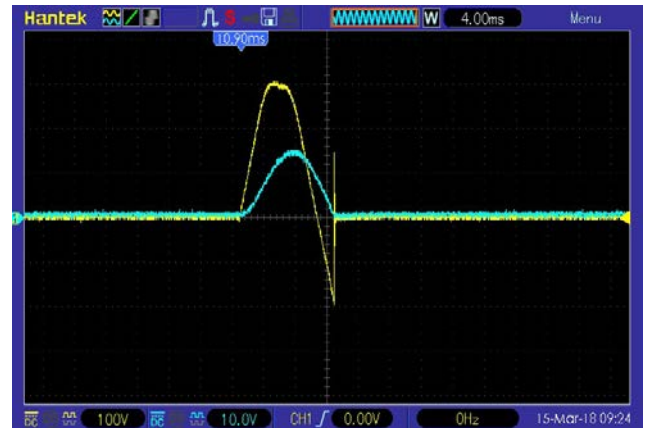
Figure 11. Load disconnection upon the appearance of a short-circuit
