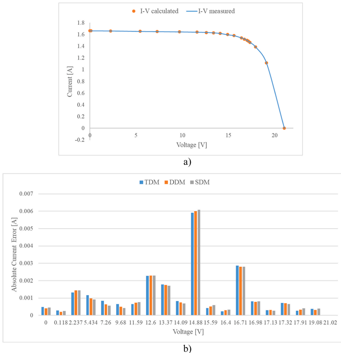
Fig. 5. STM6-40 monocrystalline photovoltaic panel: a) Comparison between I-V characteristics measured and calculated using HSDA algorithm for TDM model; b) Absolute current errors for HSDA algorithm in the cases TDM, DDM, and SDM models.
