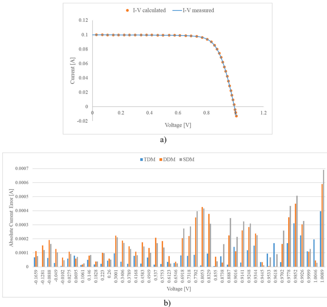
Fig. 7. PVM_752GaAs photovoltaic panel: a) Comparison between I-V characteristics measured and calculated using HSDA algorithm for TDM model; b) Absolute current errors for HSDA algorithm in the cases TDM, DDM, and SDM models.
