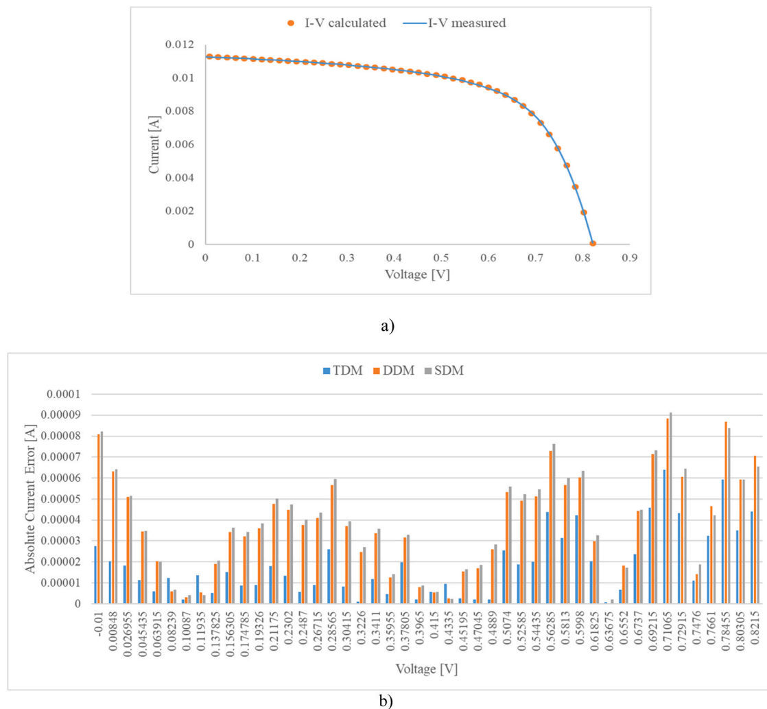
Fig. 3. aSi photovoltaic cell: a) Comparison between I-V characteristics measured and calculated using HSDA algorithm for TDM model; b) Absolute current errors for HSDA algorithm in the cases TDM, DDM, and SDM models.
