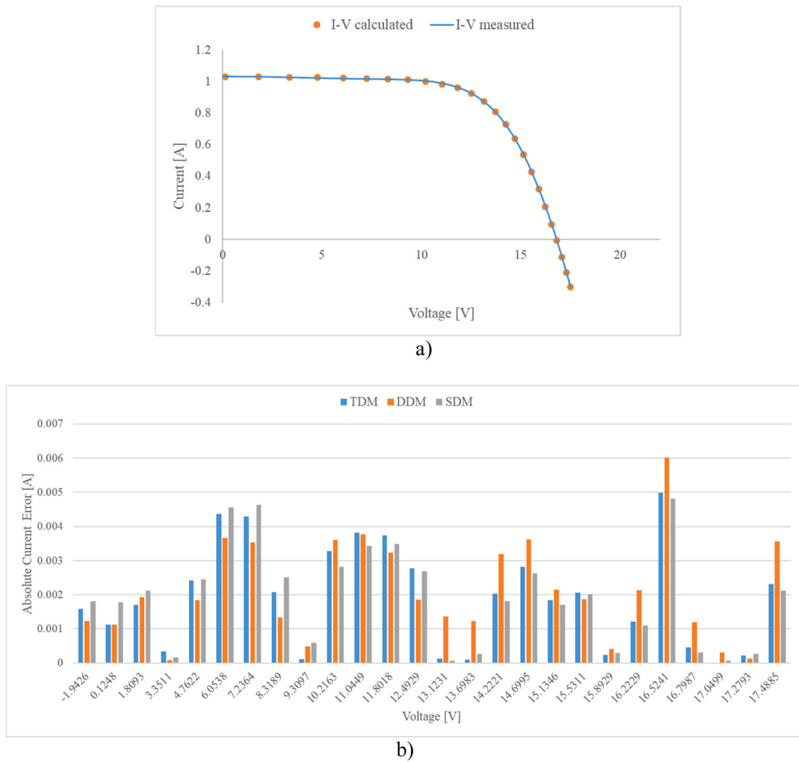
Fig. 4. PWP201 polycrystalline photovoltaic panel: a) Comparison between I-V characteristics measured and calculated using HSDA algorithm for TDM model; b) Absolute current errors for HSDA algorithm in the cases TDM, DDM, and SDM models.
