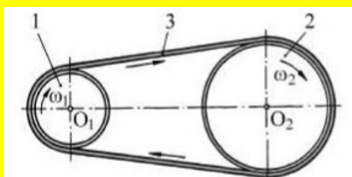
Fig.3. Belt transmission: 1-driving wheel, 2-driven wheel, 3- trapezoidal belt (V-belt);
