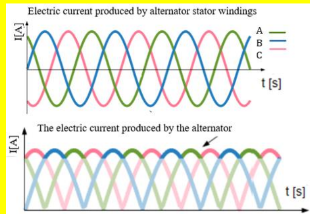
Fig.8. The electric current produced by the car alternator.
