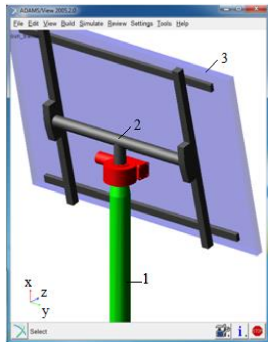
Figure 1. The MBS model of the mono-axial azimuthally sun tracker.
