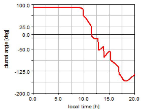
Figure 6. The control law for the diurnal motion.
