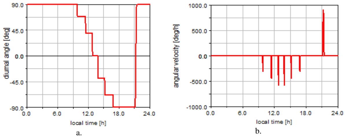
Figure 3. The tracking law for the PV system with fixed base.
