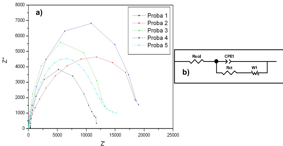
Figure 6. Niquist plot (a) and equivalent circuit for spectra modelation (b)
