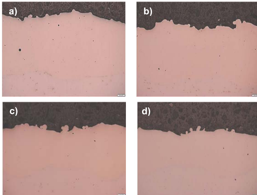
Figure 2. OM of laser clad coatings (a) Sample 1; (b) Sample 2; (c) Sample 3; (d) Sample 4.
