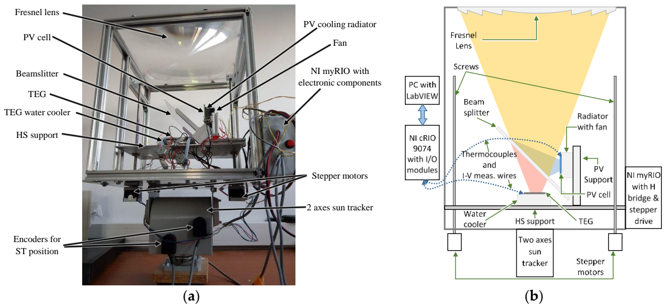
Figure 2. (a) The system setup; (b) schematic of the experimental setup.
