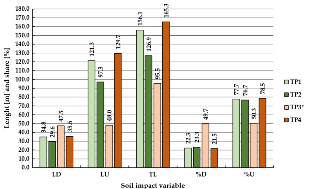
Fig. 7 Summary statistics characterizing soil disturbance Legend: TP1–TP4 stand for test plots 1–4, LD—length on which soil disturbance was observed, LU—length on which the soil was found to be undisturbed, TL—total length, %D: share of disturbed soil, %U: share of undisturbed soil. *denotes significant differences in terms of soil disturbance when compared to each other test plot
