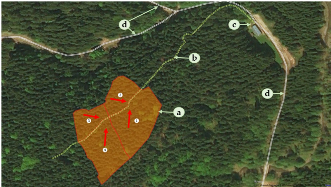
Fig. 1 Study area showing the four delimited test plots, the skidding road used for extraction, location of the landing and the main forest road network in the area. Legend: a : area of study, delimited from the forest compartment, where 1 is the test plot 1 (TP1), 2—test plot 2 (TP2), 3—test plot 3 (TP3) and 4—test plot 4 (TP4); b : skidding road
