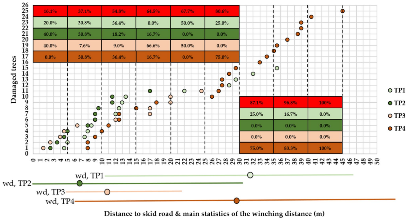
Fig. 4 Absolute and relative distribution of damaged trees in relation to their distance to the skidding road. Legend: TP1–TP4 stand for the test plots 1–4, figures given in red boxes stand for the global shares in relation to the distance to the skidding road, figures given in light and dark green and brown boxes stand for the shares of damaged trees
