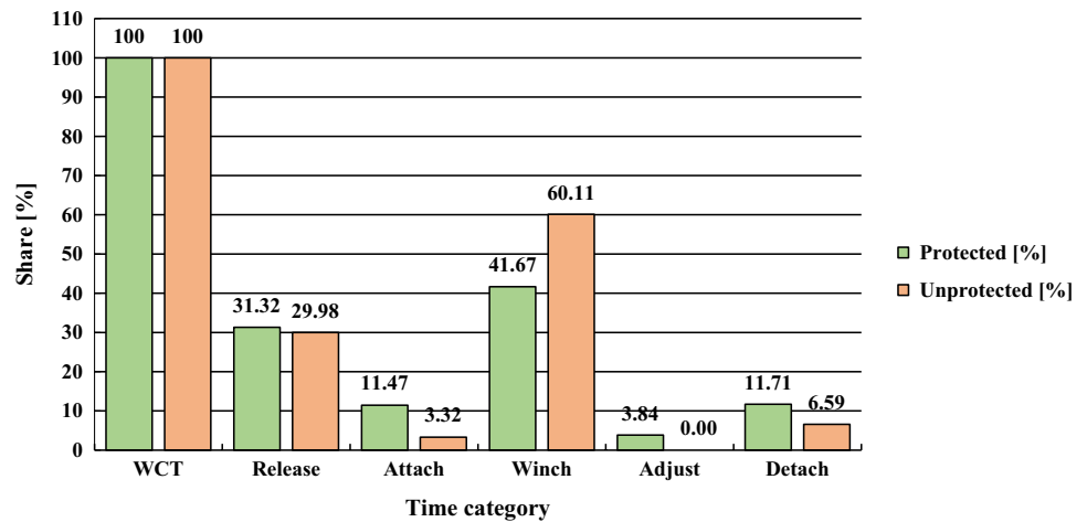
Fig. 8 Share of time consumption on work elements and main treatments. Legend: protected refers to the data collected in TP1 and TP2, unprotected refers to the data collected in TP3 and TP4
