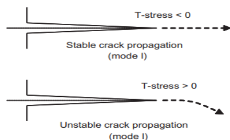
Figure 1. The stability of the crack propagation as a function of T .
