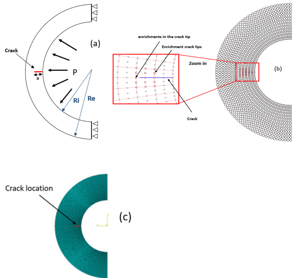
Figure 5. Geometry construction: (a) crack size ranges from 0.2 to 0.45, (b) mesh for X-IGA, (c) mesh used for X-FEM.
