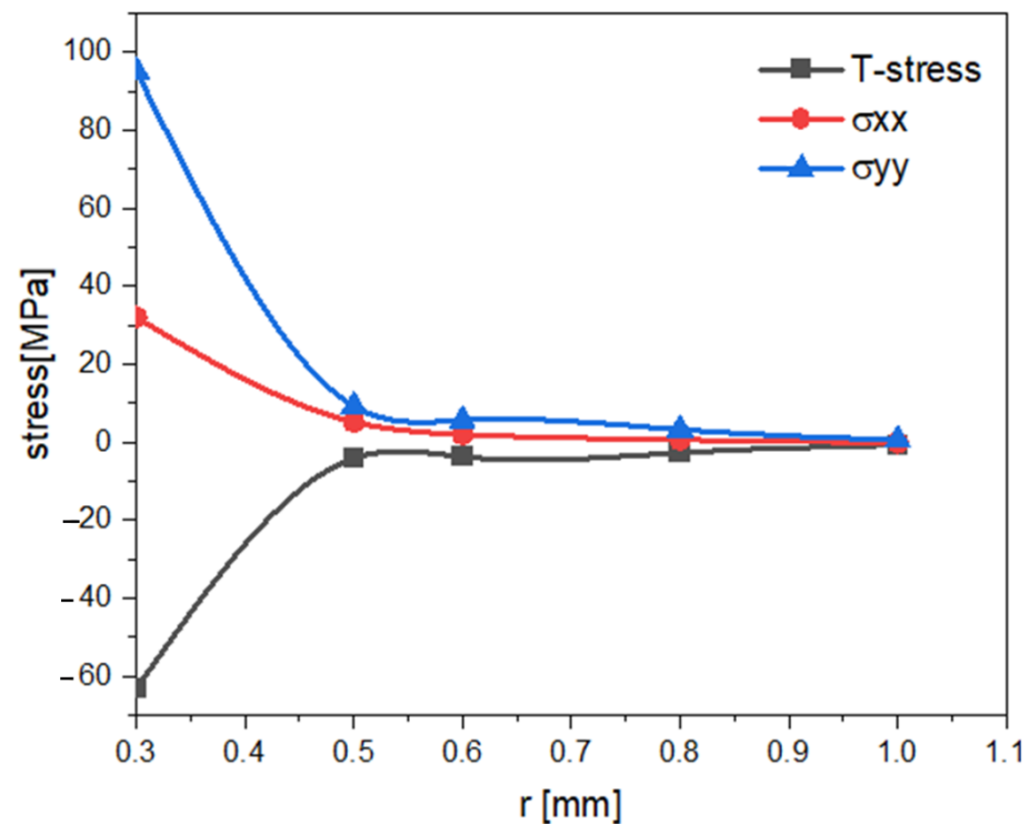
Figure 7. T-Stress as a function of r computed by X-IGA.
