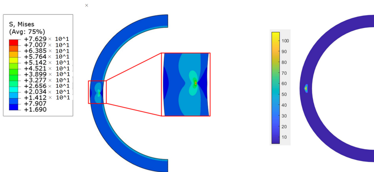
Figure 6. The distribution of Von Mises stress with X-FEM on the right and X-IGA on the left .
