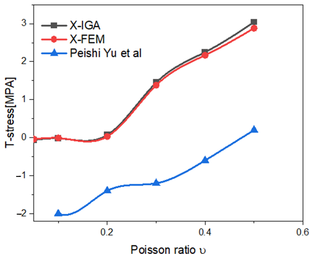
Figure 10. Variation of T -stress with Poisson ratio, by X-FEM and X-IGA.
