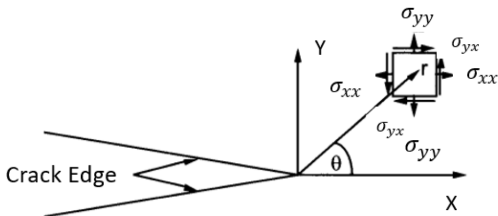
Figure 4. Crack tip coordinate [20].
