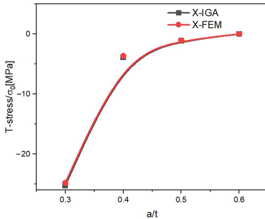
Figure 8. The variation of T\text{-stress}/\sigma_0 as function a/t .
