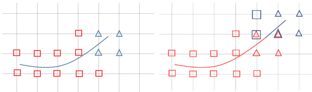
Figure 3. Steps in the enrichment method; when the crack propagates, enrichment at the crack front becomes discontinuous enrichment, and nodes (not enriched) become enriched [32].
