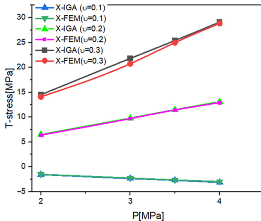
Figure 9. T\text{-stress} as a function of internal pressure, for different values of Poisson's ratio.
