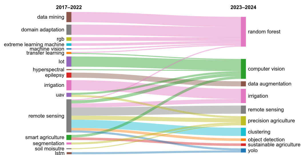
Figure 3. Authors’ keywords from all documents retrieved through the search query on the Web of Science, after excluding terms related to the search query, visualized using the thematic evolution function of the bibliometrix R package (version 4.3.0).
