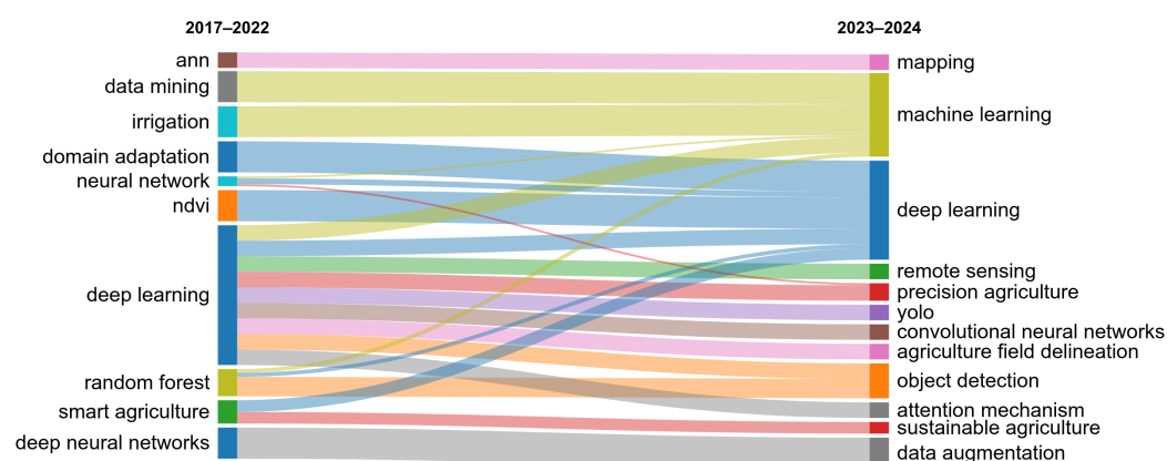
Figure 2. Authors’ keywords from all documents retrieved through the search query on the Web of Science, visualized using the thematic evolution function of the bibliometrix R package (version 4.3.0).
