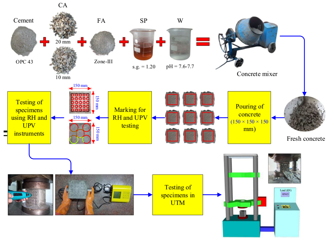
Figure 3. Preparation of specimens (casting, marking, NDT and compression testing).
