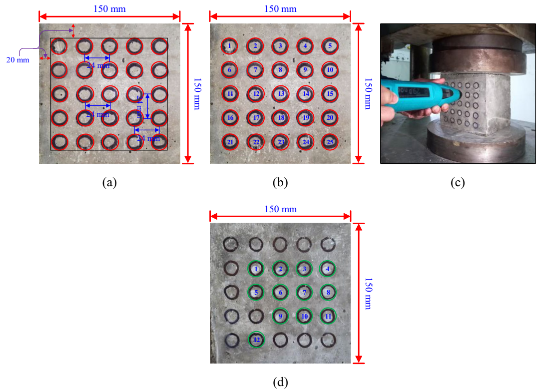
Figure 4. Concrete cubes (a) Marking of 15 mm circle for RH test (b) Assigning number to each circle and (c) Impression of RH test.
