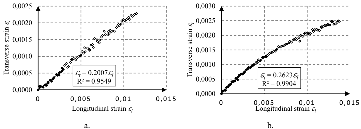
Figure 8. Transverse strain related \varepsilon_t to longitudinal strain \varepsilon_l in case of the Jute / glass / epoxy composite material: a. Specimen 1; b. Specimen 5.
