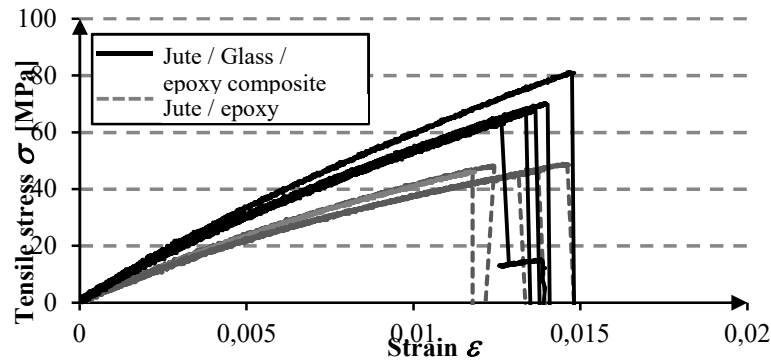
Figure 6. Stress-strain ( \sigma - \varepsilon ) curves recorded in tensile test in case of the composite materials tested.
