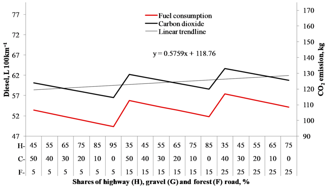
Figure 5. Effects of road-network setups on CO 2 emissions of 76 t vehicle in 52% backhauling transportation of renewable wood.
