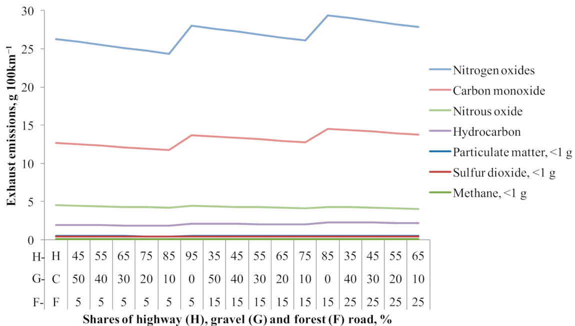
Figure 4. The effect of road-network setup on exhaust emissions of 76 t vehicles in line-hauling transportation of renewable wood.
