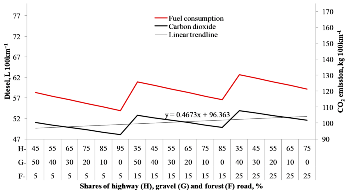
Figure 7. Effects of road-network setups on CO 2 emissions of 76 t vehicle in 70% backhauling transportation of renewable wood.
