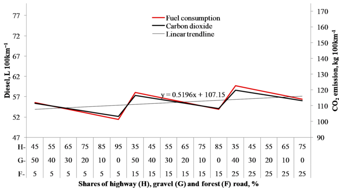
Figure 6. Effects of road-network setups on CO 2 emissions of 76 t vehicle in 60% backhauling transportation of renewable wood.
