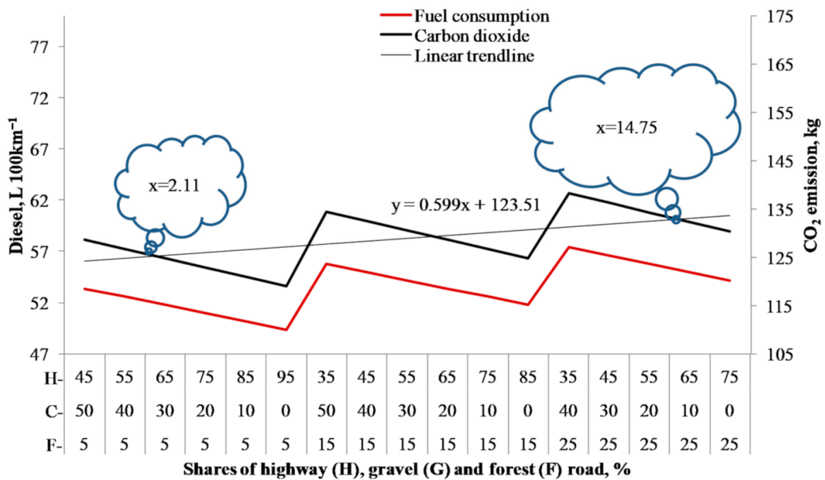
Figure 2. The effect of road-network setup on CO 2 emissions of 76 t vehicles in line-hauling transportation of renewable wood.
