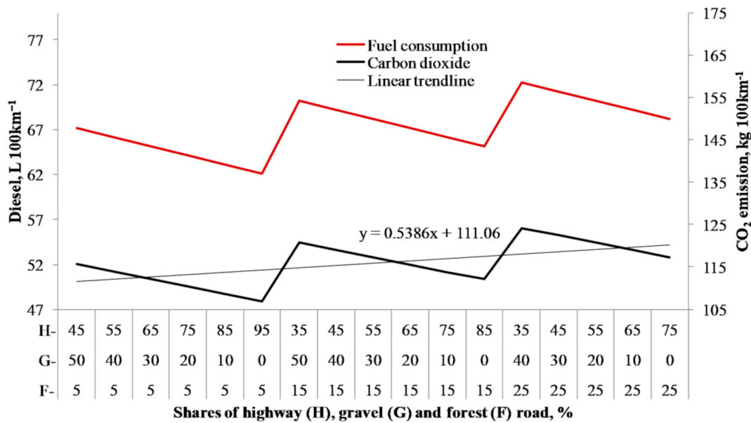
Figure 10. Effects of road-network setups on CO 2 emissions of 92 t vehicle in 70% backhauling transportation of renewable wood.
