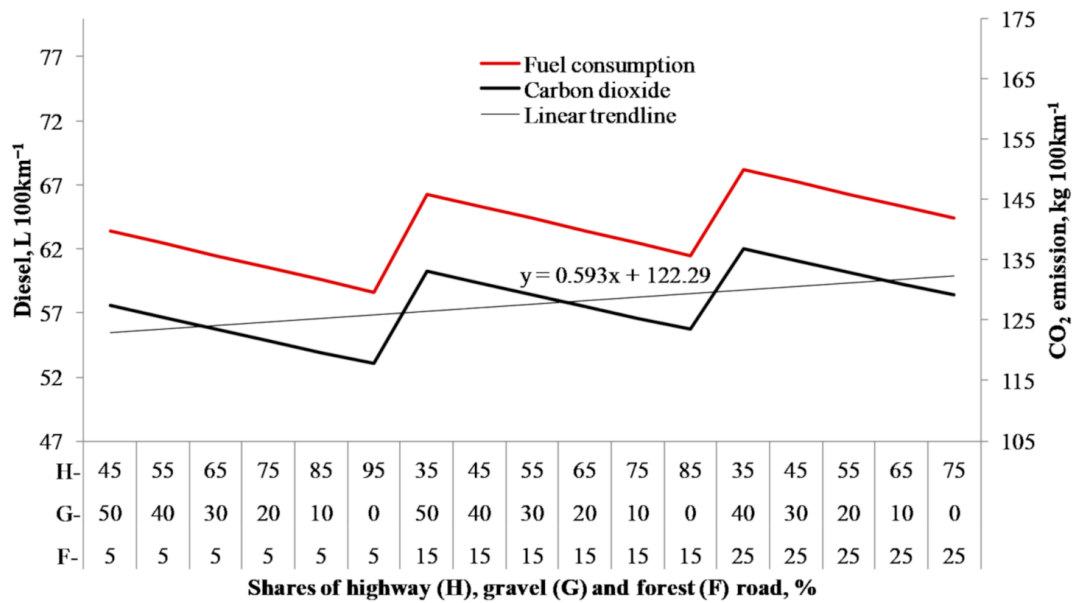
Figure 9. Effects of road-network setups on CO 2 emissions of 92 t vehicle in 60% backhauling transportation of renewable wood.
