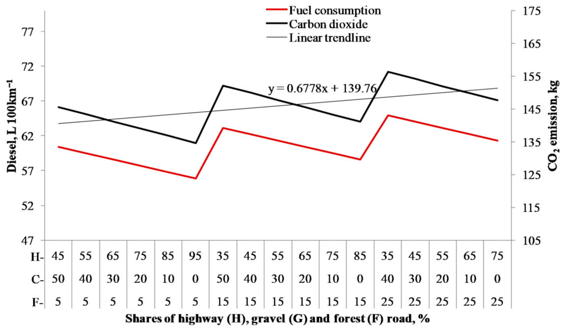
Figure 3. The effect of road-network setup on CO 2 emissions of 92 t vehicles in line-hauling transportation of renewable wood.
