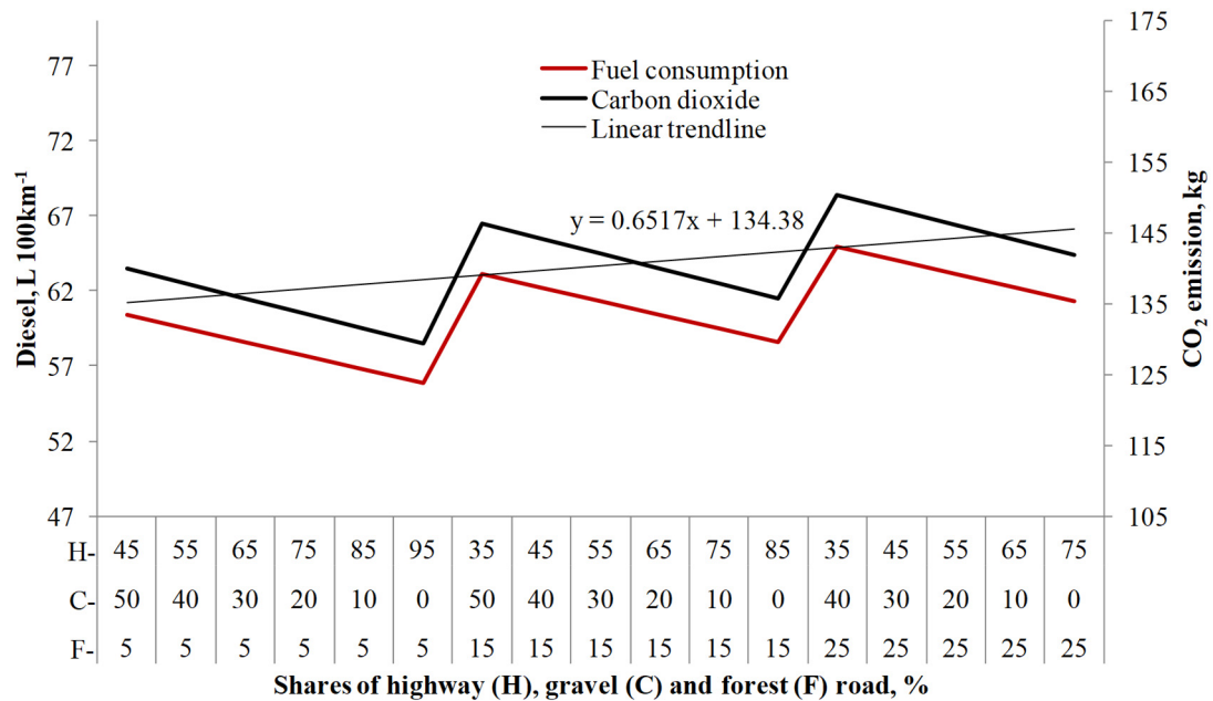
Figure 8. Effects of road-network setups on CO 2 emissions of 92 t vehicle in 52% backhauling transportation of renewable wood.
