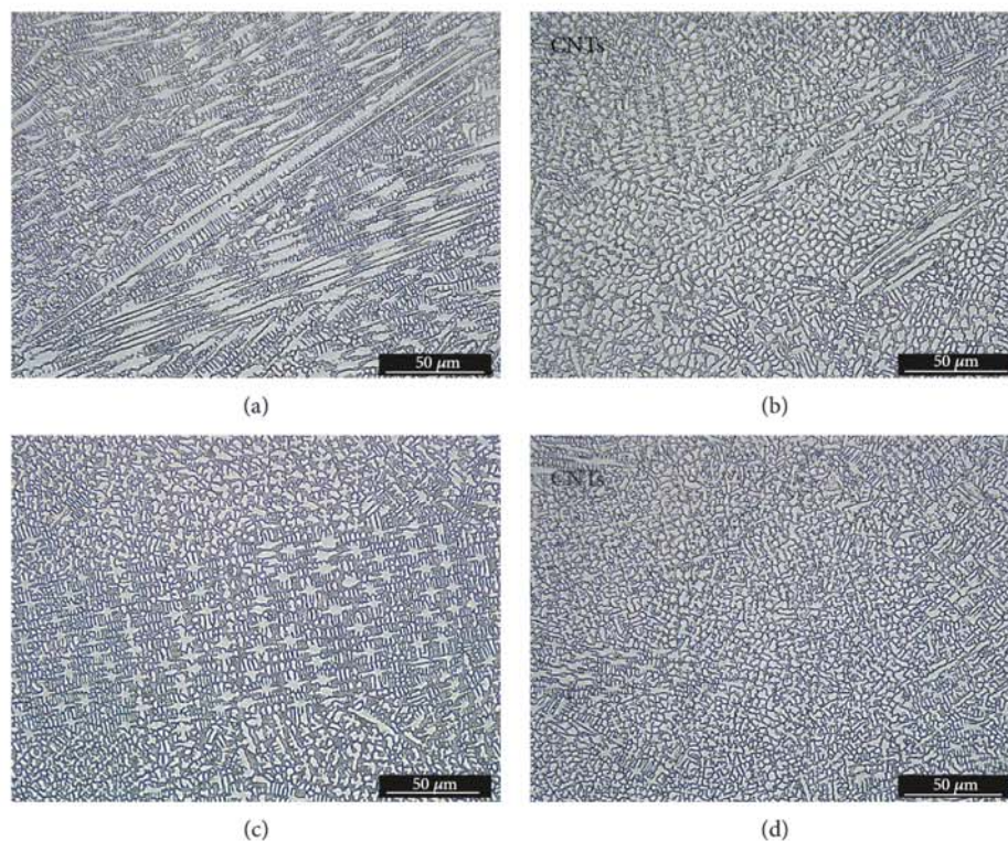
FIGURE 7: Microstructure of the machined top surface: (a, c) reference sample and (b, d) CNT composite coating.
