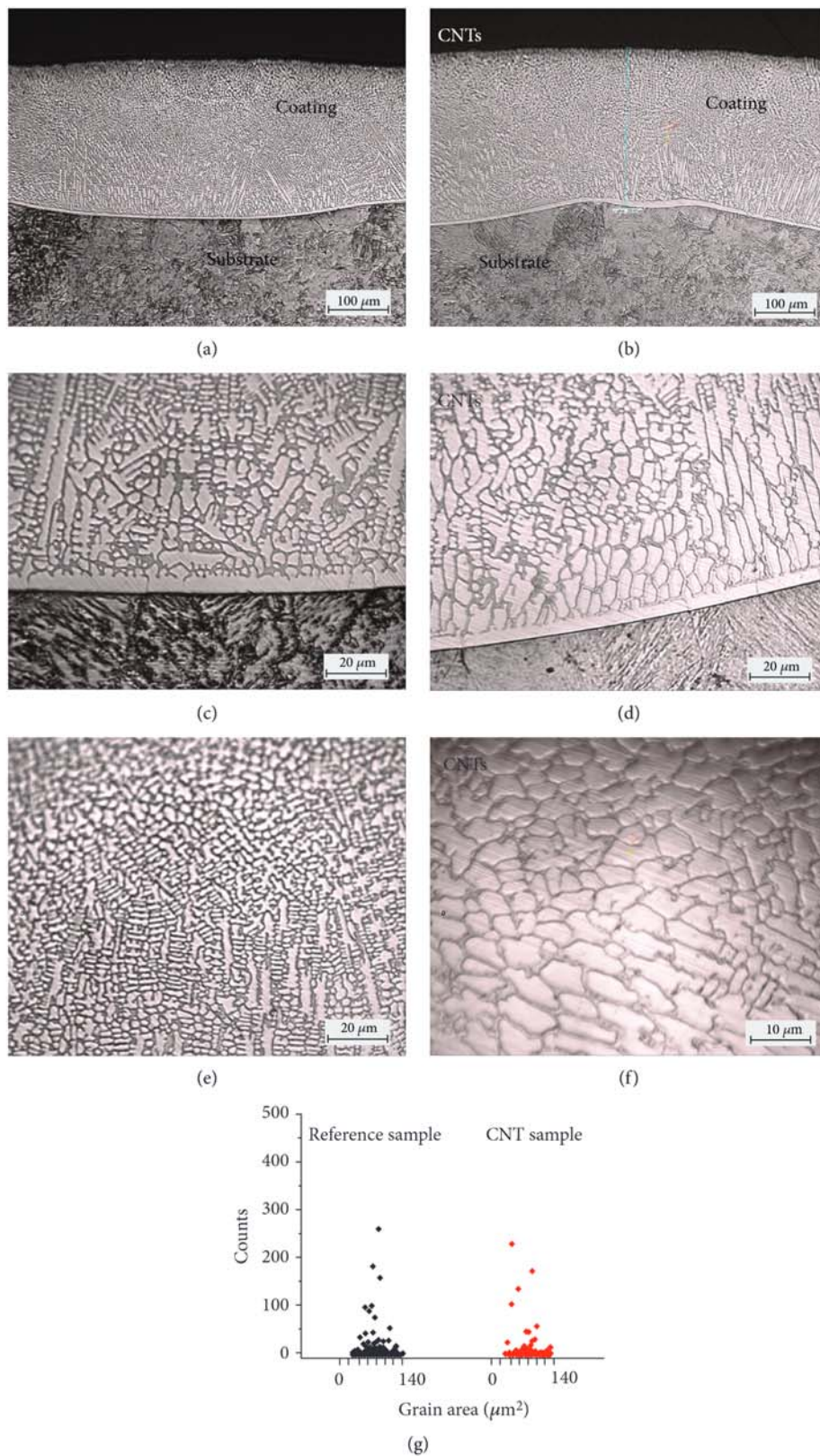
FIGURE 3: Cross-section microscopy of the clad layer of reference sample 1 (a, c, e) and of sample 2 with CNT addition (b, d, f); (g) show the grain area distribution histograms.
