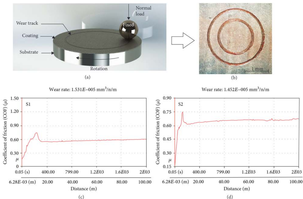
FIGURE 14: Wear results: (a) schematic representation of the ball on disk testing, (b) wear tracks on the surface of sample 1, and (c, d) plot of COF vs. distance of sample 1 and sample 2.
