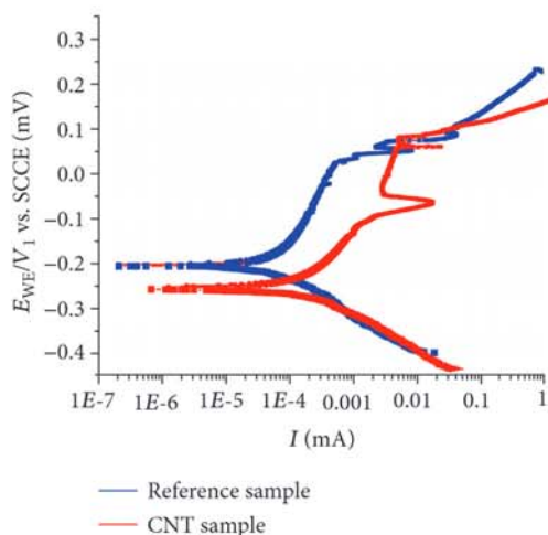
FIGURE 13: Polarization curves of the reference sample (sample 1) and of the CNT sample (sample 2).
