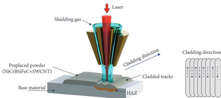
FIGURE 2: Principle of preplaced laser cladding of NiCrBSiFeC/CNT powder.
