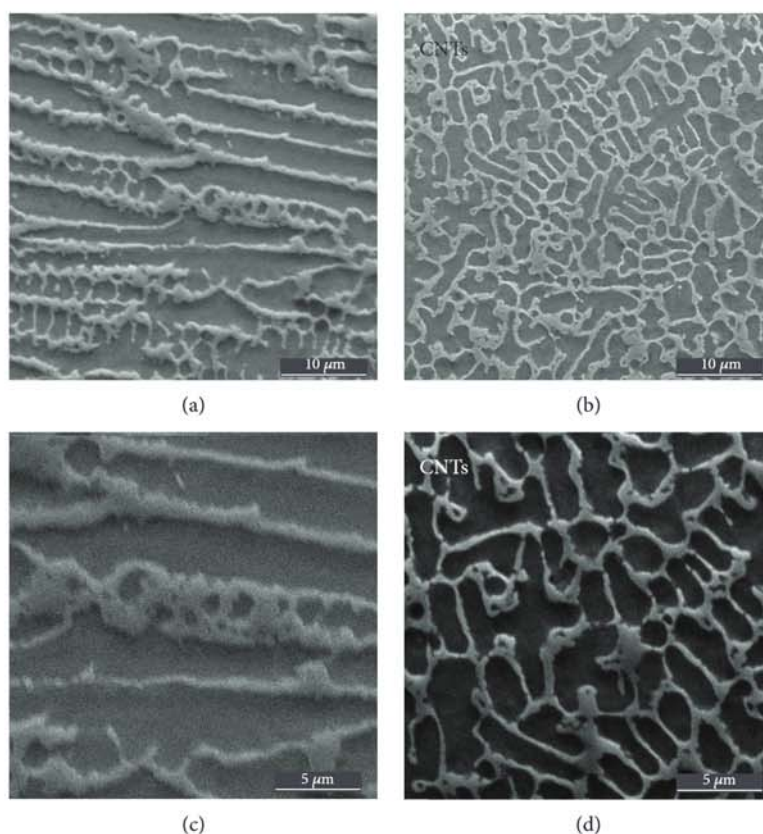
FIGURE 8: SEM microscopy of the machined top surface: (a, c) reference sample and (b, d) CNT composite coating.
