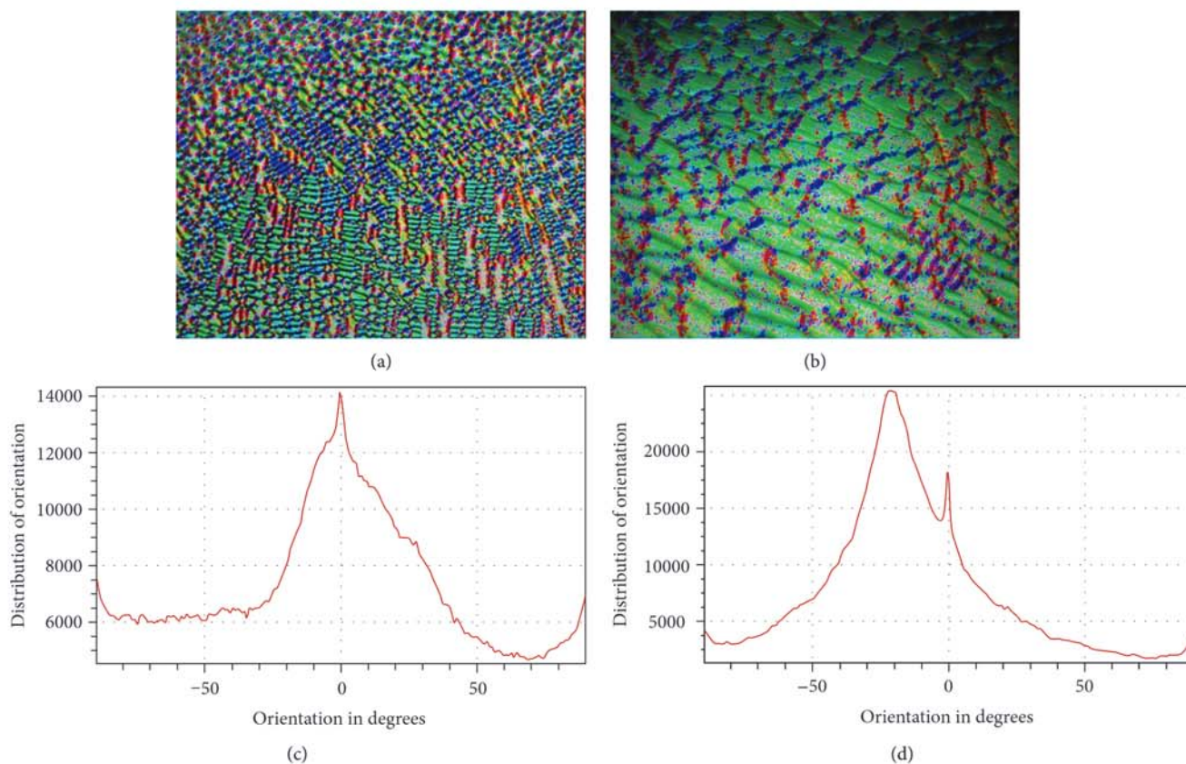
FIGURE 5: Grain orientation angle mapping and plot (obtained by ImageJ software—OrientationJ plugin).
