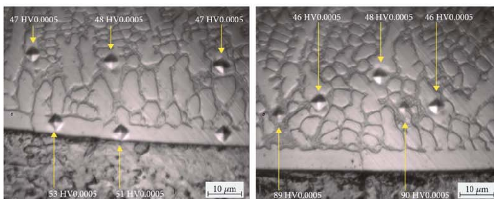
FIGURE 11: Microindention on the dendrite arm and on the interdendrite area of the cross-section of sample 1, loads 0.0005 kgf.
