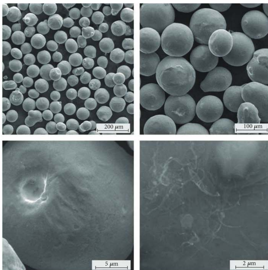
FIGURE 1: SEM micrographs at different magnifications of NiCrBSiFeC powder milled with SWCNT.
