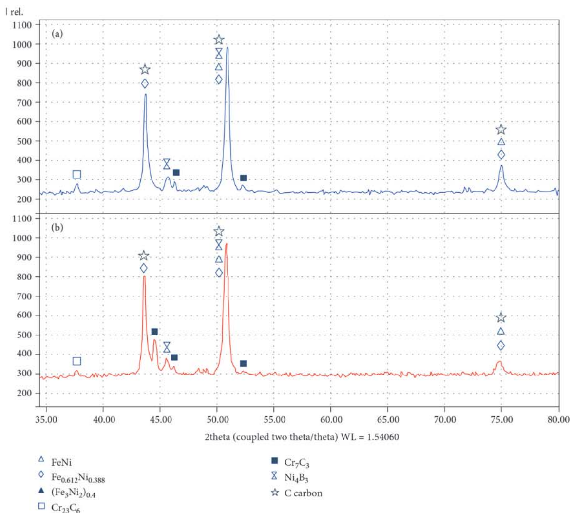
FIGURE 10: XRD diffractogram of the reference sample (a) and CNT composite coating (b).
