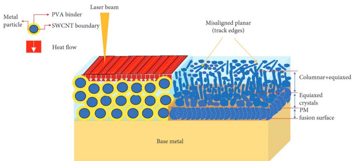
FIGURE 4: Schematic representation of the growth mechanism of a dendrite structure.
