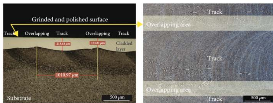
FIGURE 6: Top surface profile of the reference sample after 1/3 was removed.
