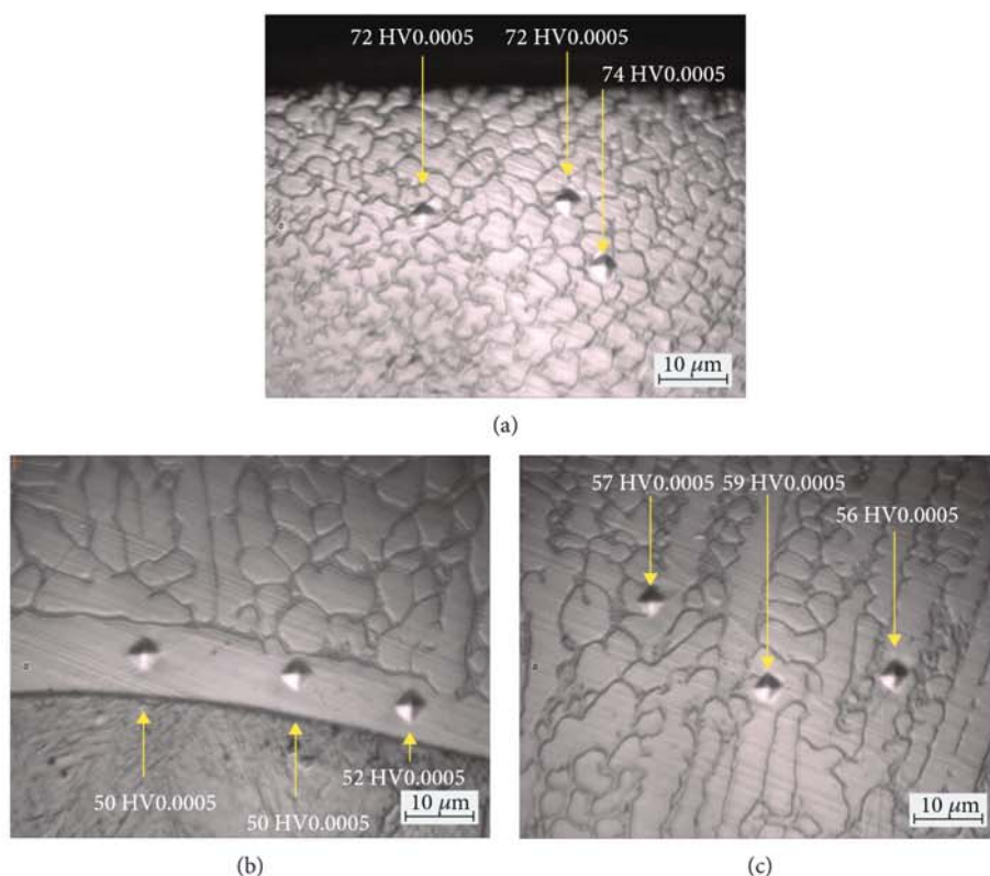
FIGURE 12: Microindention on the white dendritic formation on the cross-section of sample 2, loads 0.0005 kgf.
