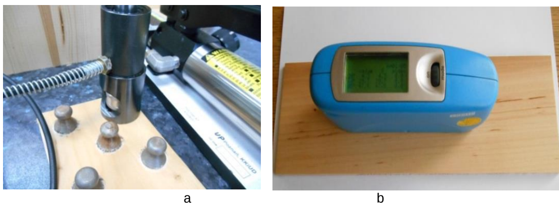
Fig. 3. PosiTest adhesion tester and dollies glued on the sample (a); PICO GLOSS 503 meter (b)
