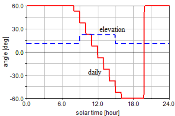
Figure 3. The angular motion functions.
