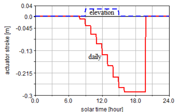
Figure 4. The linear displacements in actuators.
