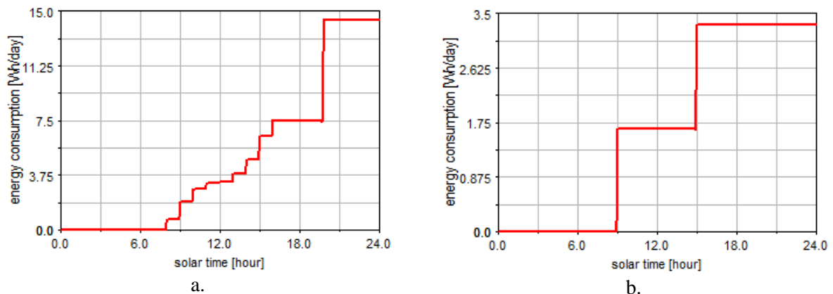
Figure 7. The energy consumptions for performing the tracking (a - daily motion, b - elevation).
