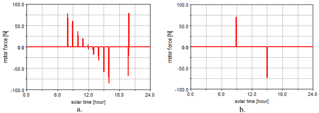
Figure 5. The motor forces generated by the linear actuators (a - daily motion, b - elevation).
