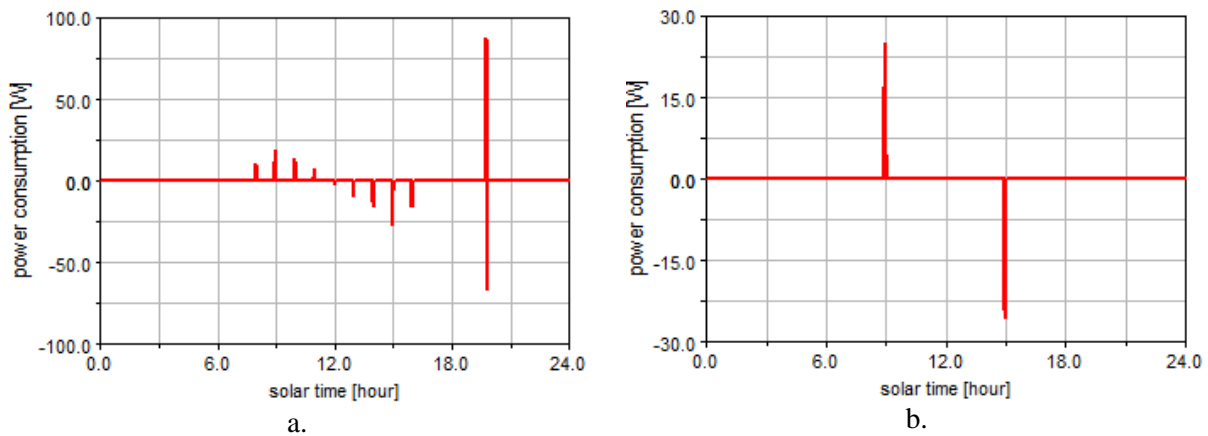
Figure 6. The power consumptions for performing the tracking (a - daily motion, b - elevation).
