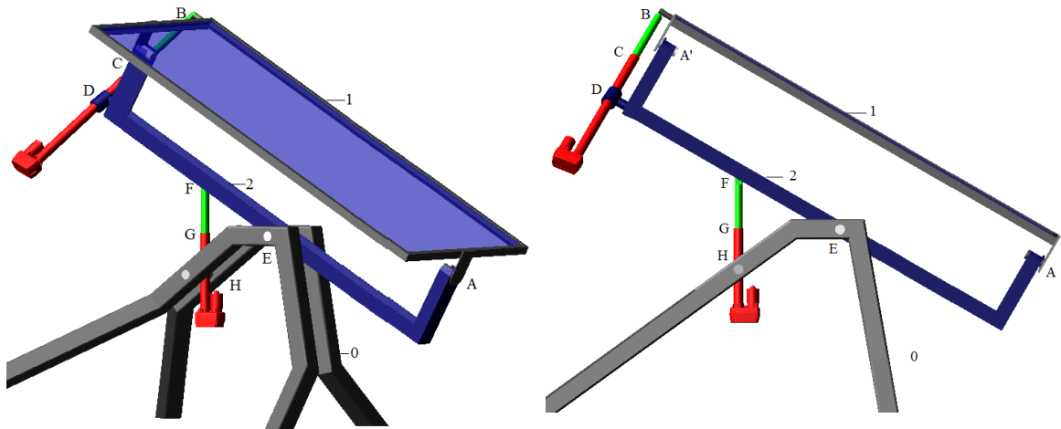
Figure 2. The MBS model of the bi-axial PV system.
