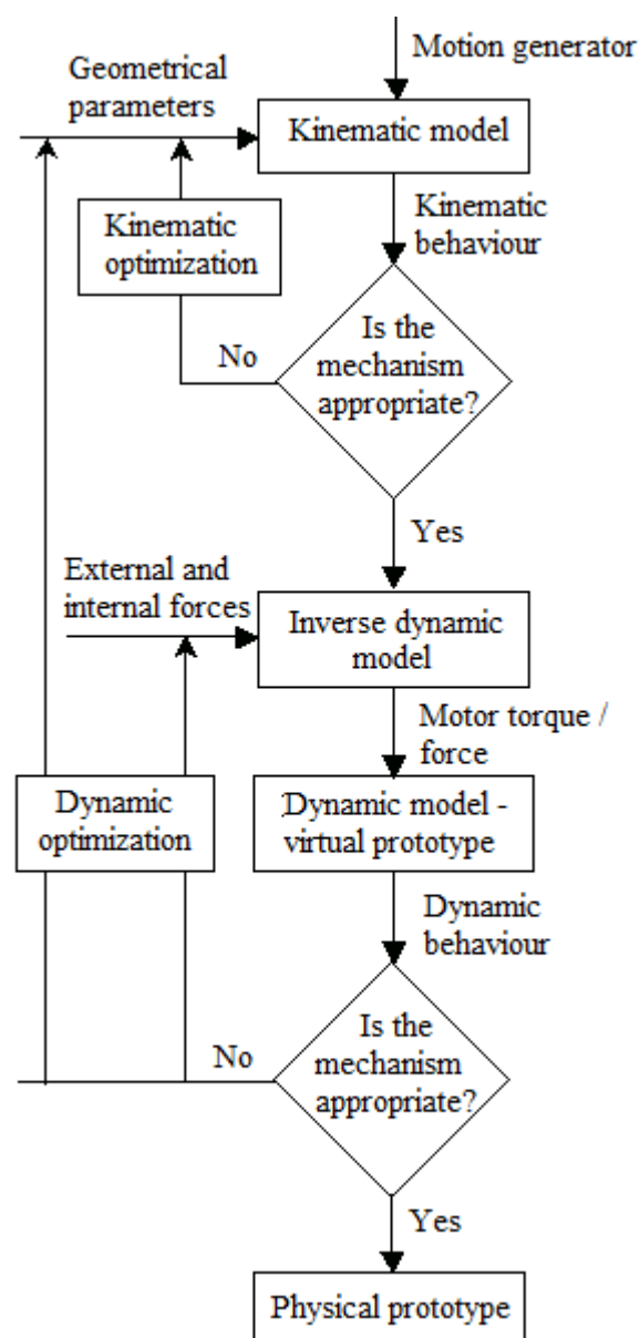
Figure 1. The designing algorithm.
