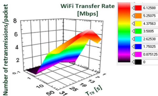
Fig. 4. The impact of Wi-Fi interferences on the number of retransmissions/packet.
