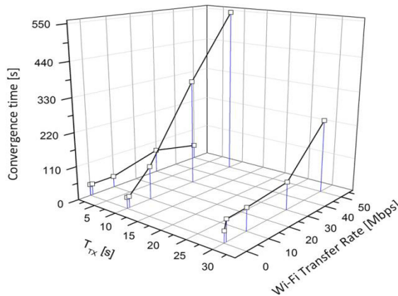
Fig. 5. The impact of Wi-Fi interferences on the hybrid network's convergence time.
