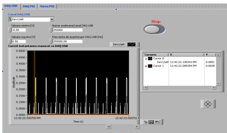
Fig. 1. The GUI of the LabVIEW automated measurement application.
