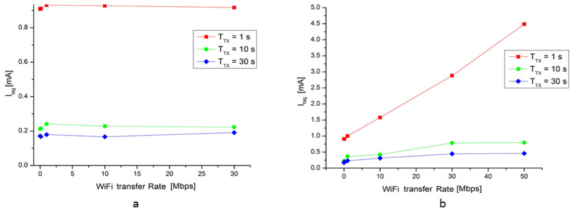
Fig. 3. (a) The energy impact of Wi-Fi interferences in the best case scenario (frequency bands not overlapping); (b) The energy impact of Wi-Fi interferences in the worst case scenario (frequency bands overlapping).
