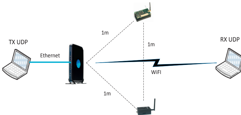
Fig. 2. Evaluation of the energy overhead of Wi-Fi induced interferences – testing scenario.
