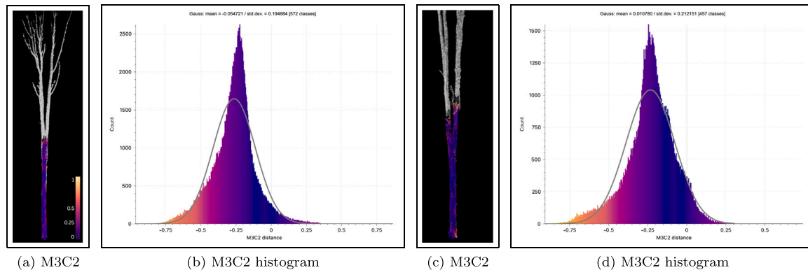
Fig. 10. Examples of the Multiscale Model-to-Model Cloud Comparison (M3C2) metric computed for two single trees, visualized in false colors. The color range used in the M3C2 point clouds in (a) and (c) is depicted in the M3C2 histograms in (b) and (d), and shown as a color bar in example (a). Blue indicates small M3C2 distances, whereas orange corresponds to large distances, i.e., considerable reconstruction errors. (For interpretation of the references to color in this figure legend, the reader is referred to the web version of this article.)
