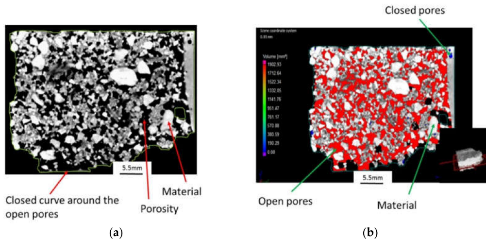
Figure 6. CT cross-sections through composite 2 of sample S1: (a) gray values indicate the material and porosity; (b) color map is used to indicate the pore volume size.
