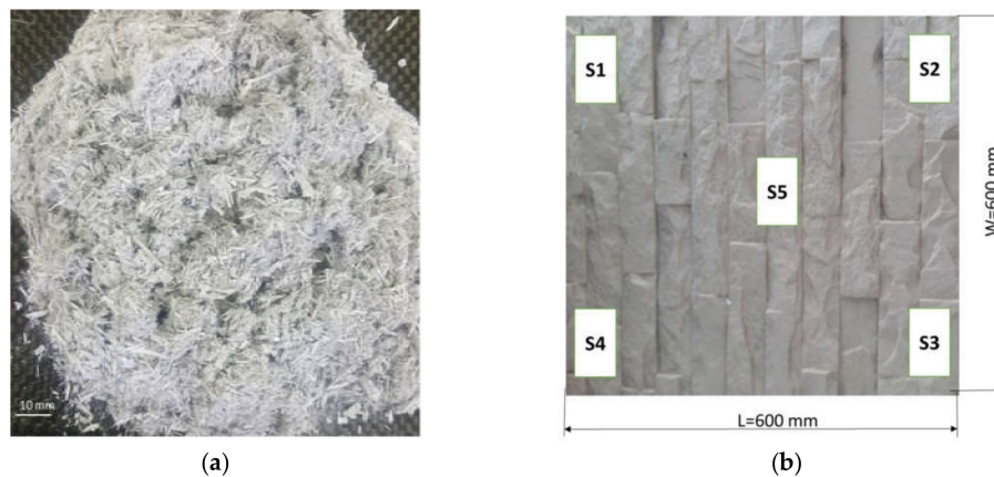
Figure 2. (a) Resultant glass fiber waste from the grinding process. (b) Scheme stating material sampling positions taken from the panels.
