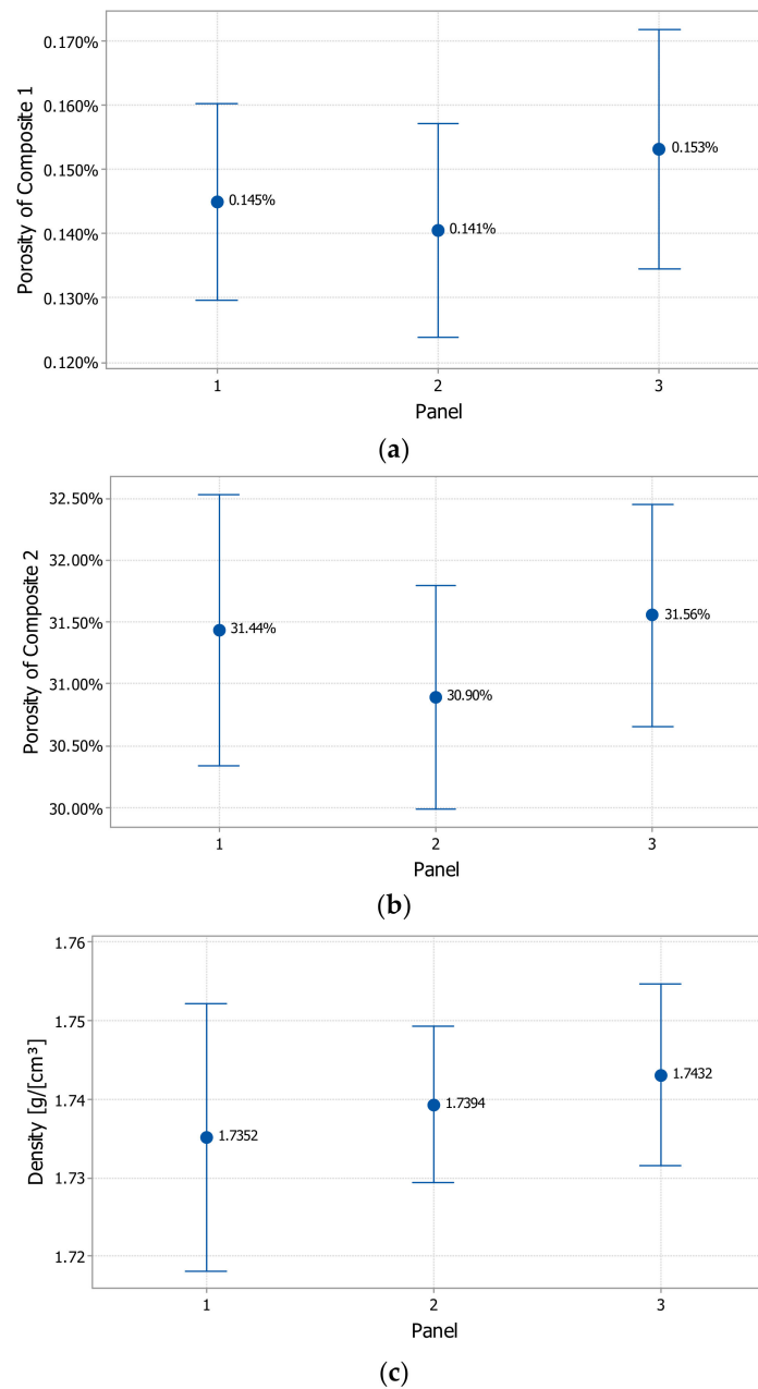
Figure 12. (a) The interval plot of the panel porosity for composite 1. (b) The interval plot of the panel porosity for composite 2. (c) The interval plot of the panel density. Bars are one standard error from the mean. Individual standard deviations were used to calculate the intervals.
