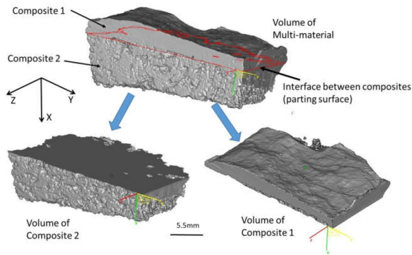
Figure 10. Splitting procedure of the multi-material volume into constituent materials volumes for sample S1. A local coordinate system is represented within the figure.
