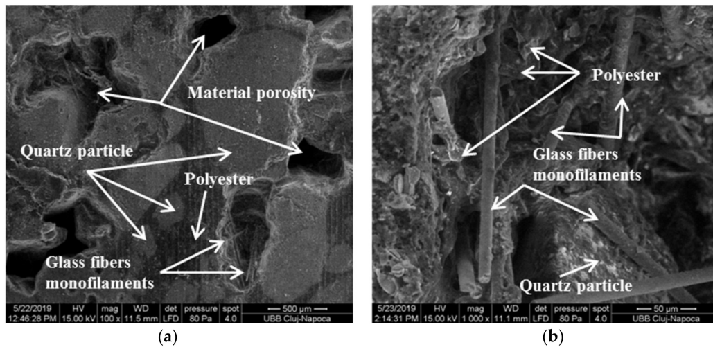
Figure 18. SEM images of composite 2: (a) 1:5 \times 10^{-4} m scale (b); 1:5 \times 10^{-5} m scale.
