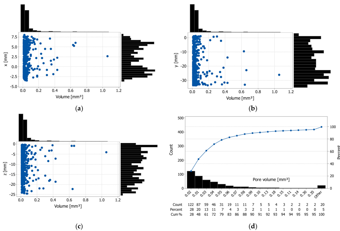
Figure 14. Closed pore volume distribution of sample S1: (a) versus X; (b) versus Y; (c) versus Z; (d) the number of pores versus pore volume.
