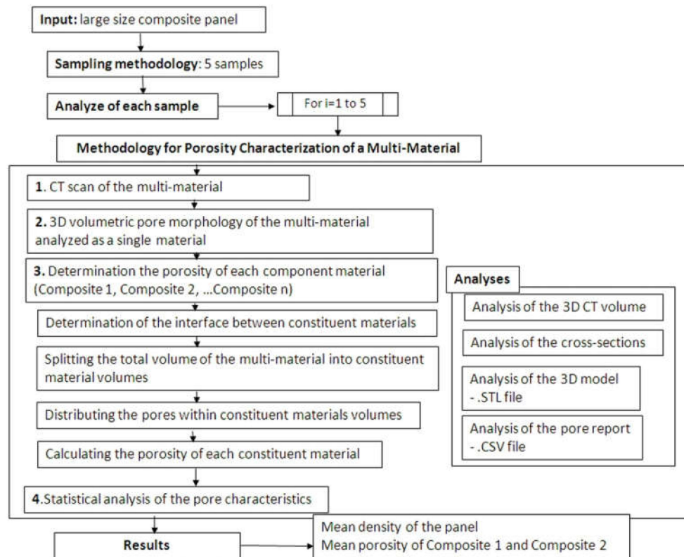
Figure 5. Methodology for porosity and density analysis of a multi-material composite.
