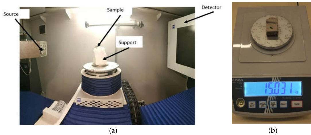
Figure 4. (a) Layout of the X-ray CT analysis. (b) Precision digital scale.
