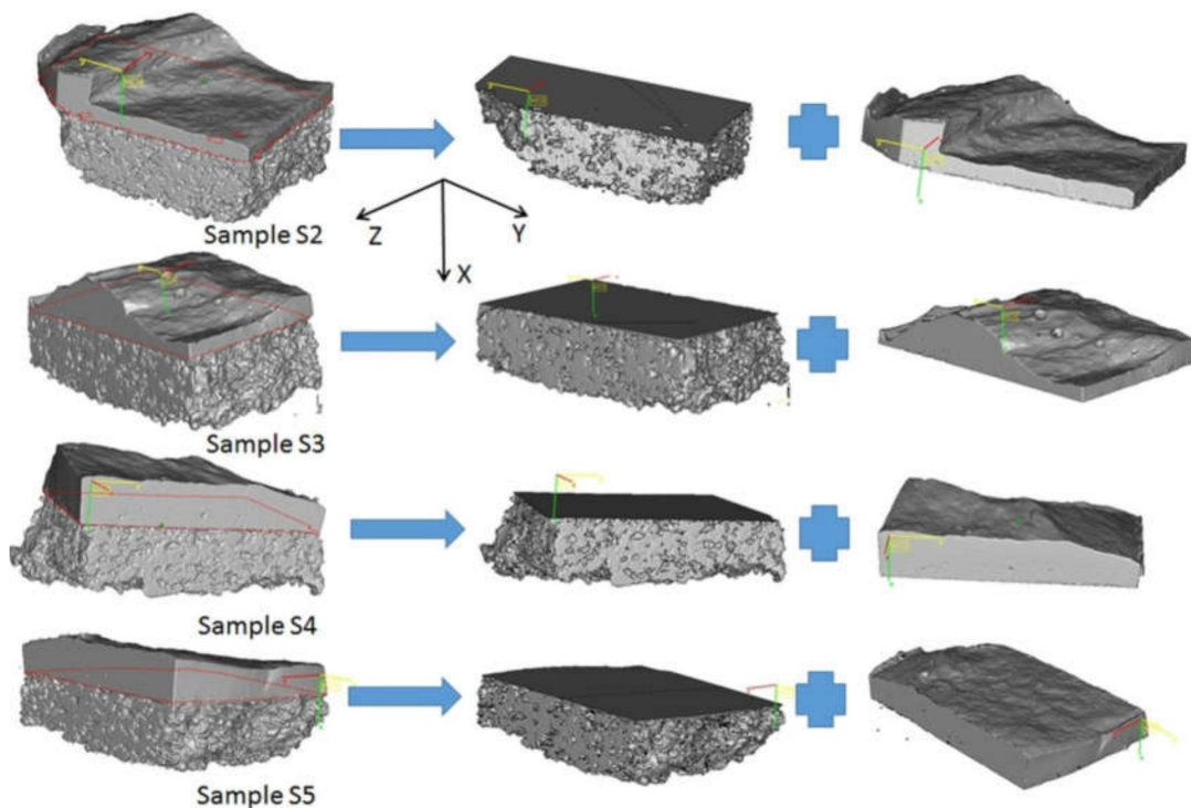
Figure 11. Visualization of the 3D stereolithography (STL) model for the multi-material composite (left column), composite 2 (middle column), and composite 1 (right column).
