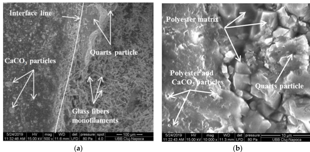
Figure 19. SEM images of the interface between composite 1 and the composite 2: (a) 1:1 \times 10^{-4} m scale; (b) 1:1 \times 10^{-5} m scale.
