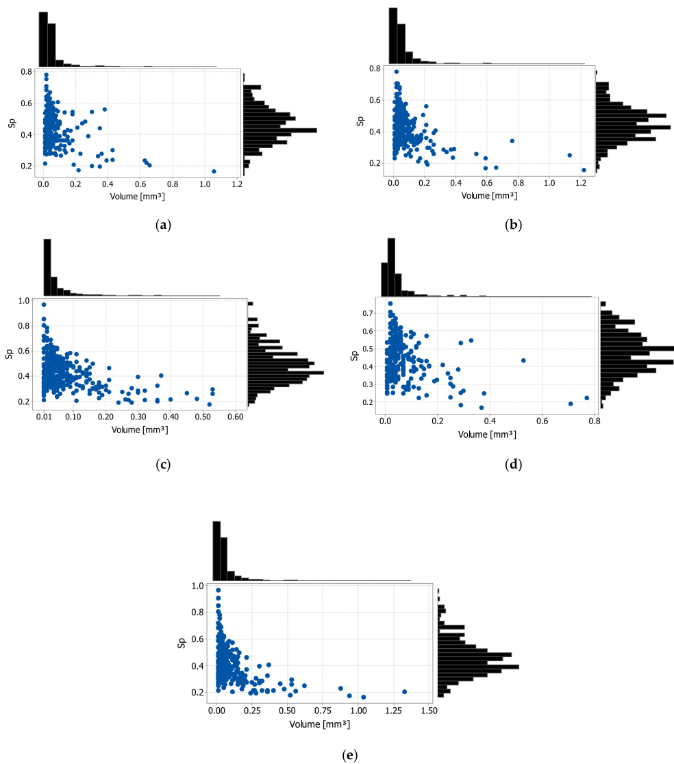
Figure 16. The sphericity ( Sp ) parameter of closed pores for: (a) sample S1; (b) sample S2; (c) sample S3; (d) sample S4; (e) sample S5.
