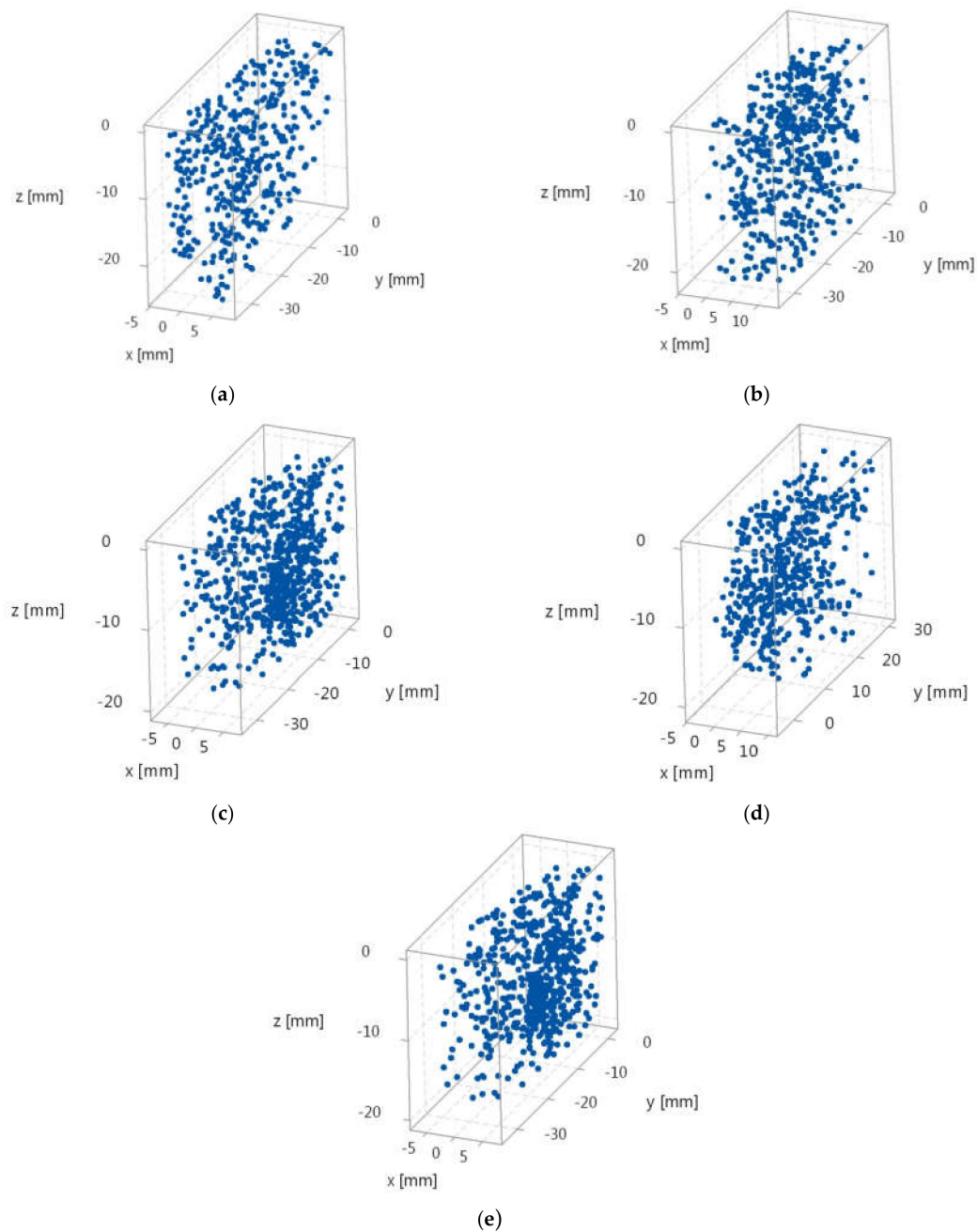
Figure 13. The 3D distribution of the pores x , y , and z are the coordinates of the circumscribed sphere center of the pore: (a) sample S1; (b) sample S2; (c) sample S3; (d) sample S4; (e) sample S5.
