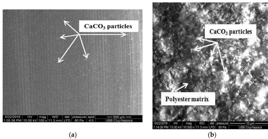
Figure 17. Scanning electron microscopy (SEM) images of composite 1: (a) 1:5 \times 10^{-4} m scale (b); 1:1 \times 10^{-5} m scale.
