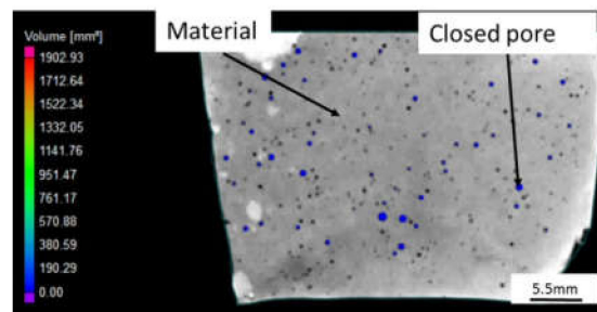
Figure 7. CT cross-section images through composite 1 of sample S1: color map is used to indicate the pore volume size.
