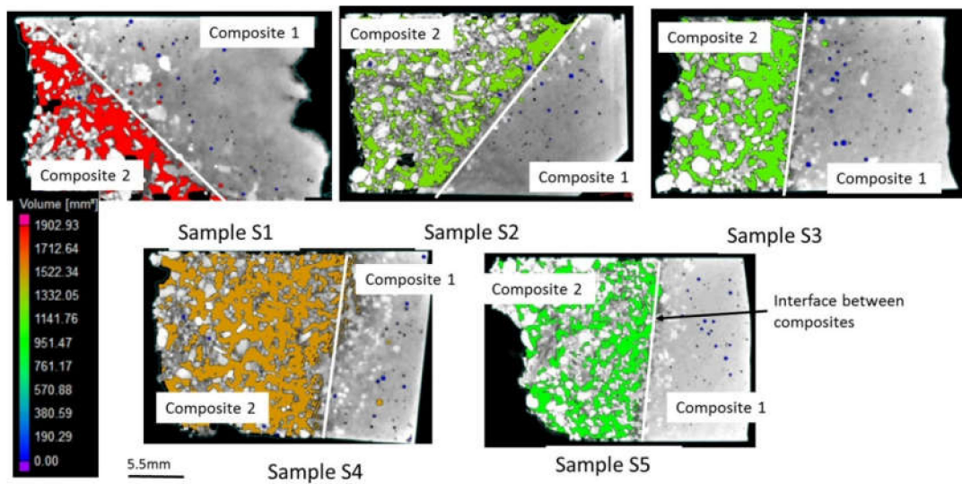
Figure 8. Representative CT cross-sections of composite 1 and composite 2, with color-coding of pore volumes for samples S1, S2, S3, S4, and S5. The color map and the scale are valid for all subfigures. The visible white lines indicate the interfaces between composites for all the samples.
