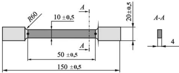
Fig. 5. Shape and dimensions of the specimens for tensile test
