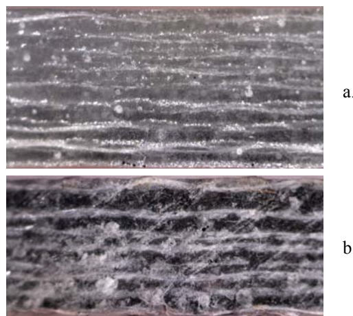
Fig. 8. Photos (by using a digital microscope) of a cross-section of the composite material: a.WE1; b. WE1R
