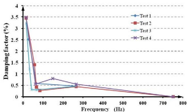
Fig. 8. Damping factor versus frequency in case of the plate made of composite WE1R
