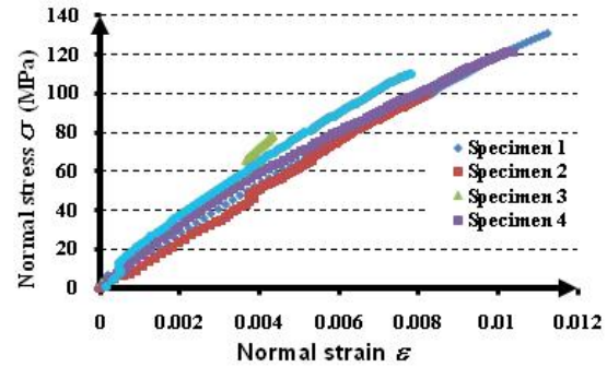
Fig. 6. Stress-strain curves ( \sigma - \epsilon ) recorded in flexural test in case of the specimens made of polyester resin
