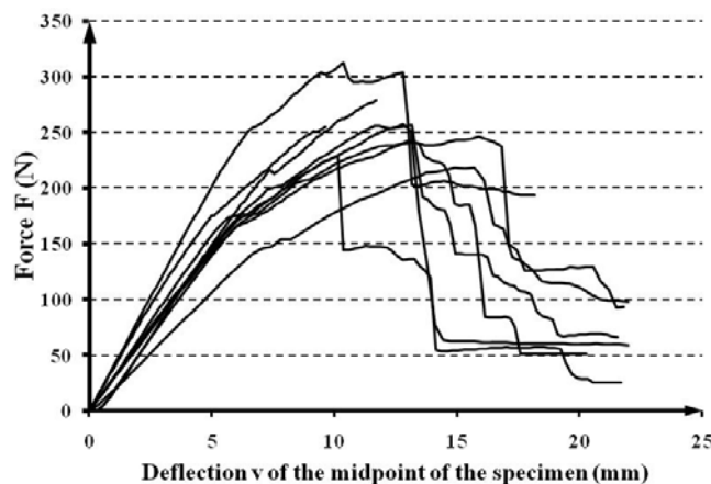
Fig. 2. F-v curves recorded in flexural test in case of the composites WE1R filled additionally with rubber
