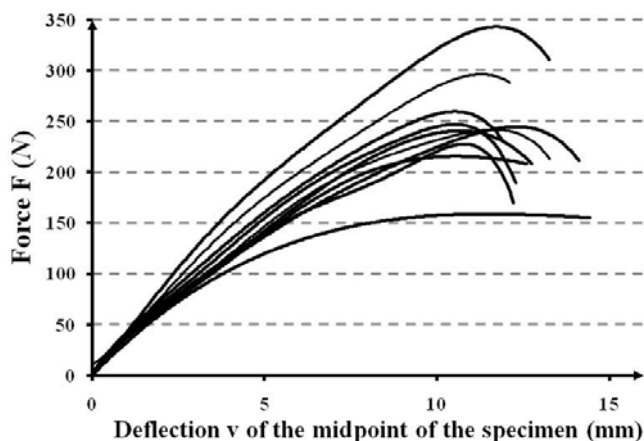
Fig. 1. F-v curves recorded in flexural test in case of the composite WE1 reinforced only with glass woven fabric
