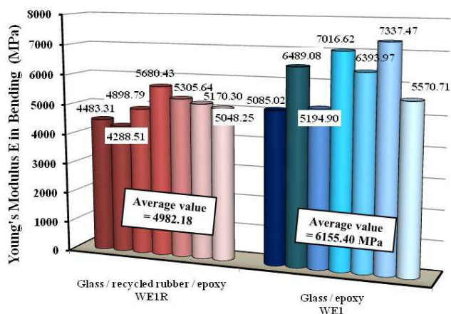
Fig. 3. Values of Young's modulus E measured in flexural test
