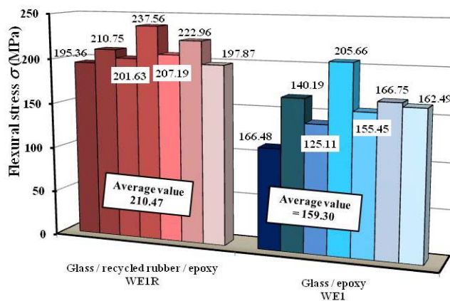
Fig. 4. Maximum values of normal stress \sigma_{\text{max}} recorded in flexural test
