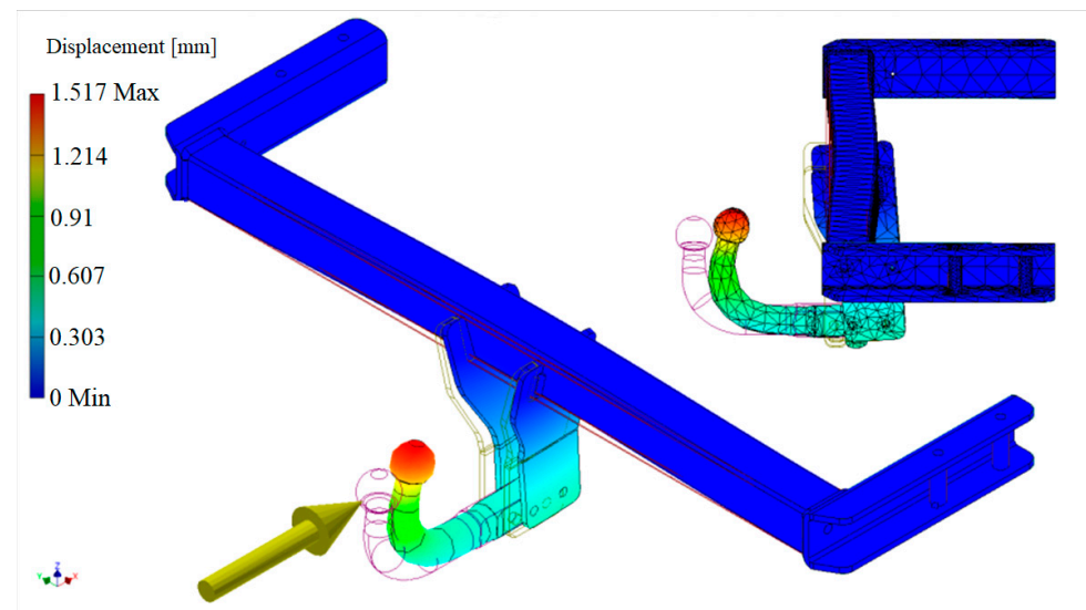
Figure 12. Displacements and (exaggerated) deformation mode of the towing system.
